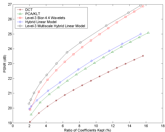
Fig. 11. Top: Comparison of several image representations for the hill image. Bottom: Comparison for the baboon image. The multi-scale hybrid linear model achieves the best PSNR among all the methods for both images.
