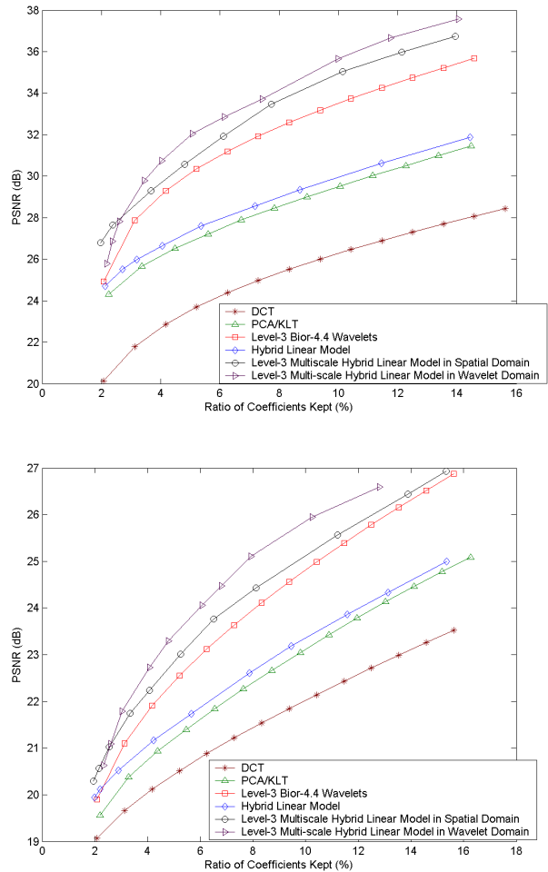
Fig. 20. Top: Comparison of several image representations for the hill image. Bottom: Comparison for the baboon image. The multi-scale hybrid linear model in the wavelet domain achieves better PSNR than that in the spatial domain.
