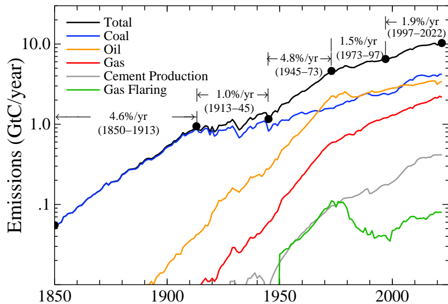
(a) Global Fossil-Fuel CO 2 Emissions
