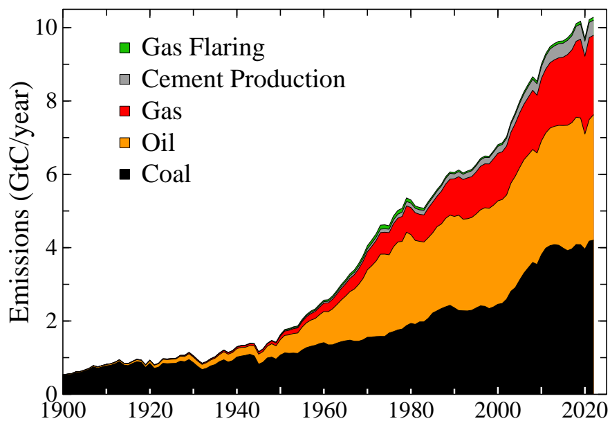
(b) Global CO 2 Emissions
