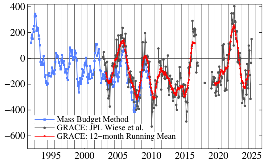
(b) Antarctica Ice Mass Change Rate
