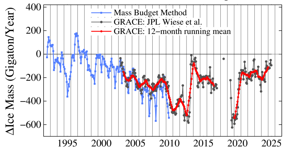
(a) Greenland Ice Mass Change Rate
