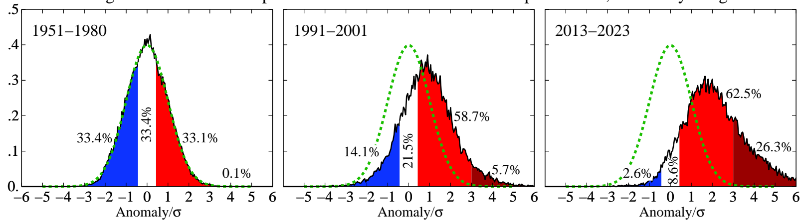
Shifting Distribution of Temperature Anomalies: Northern Hemisphere Land, June–July–August
