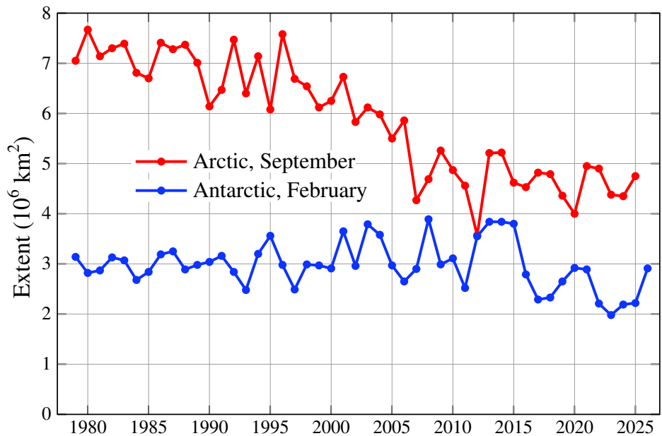
Sea Ice Extent at Minimum Months
