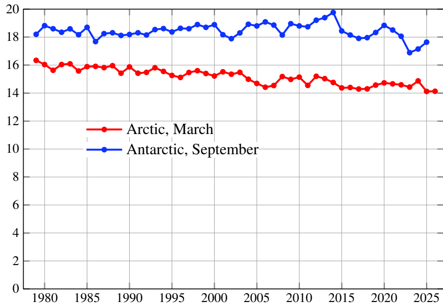
Sea Ice Extent at Maximum Months
