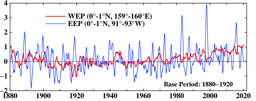
B Western and Eastern Pacific Temperature Anomalies (°C)
