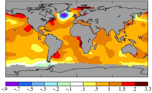
A SST Change (°C) from 1880-1920 to 2015-2019
