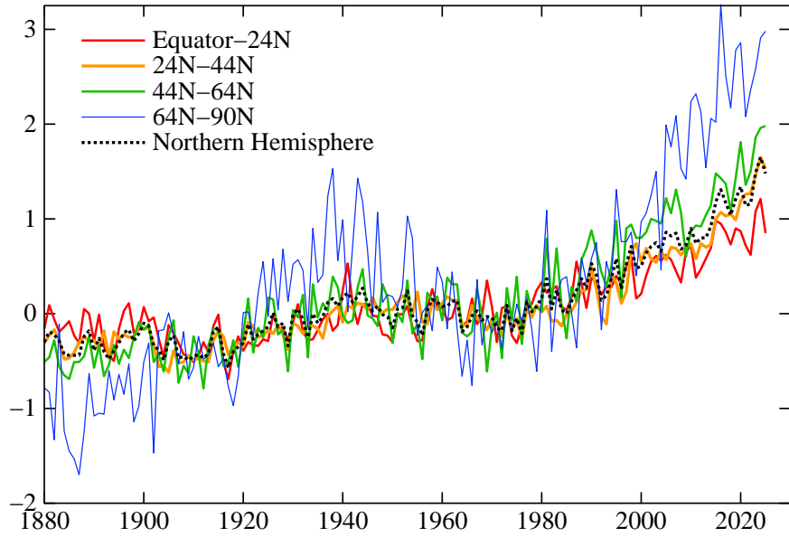
Annual Mean Surface Temperature Relative to 1951-1980 Mean (°C) in Hemispheric Zones
