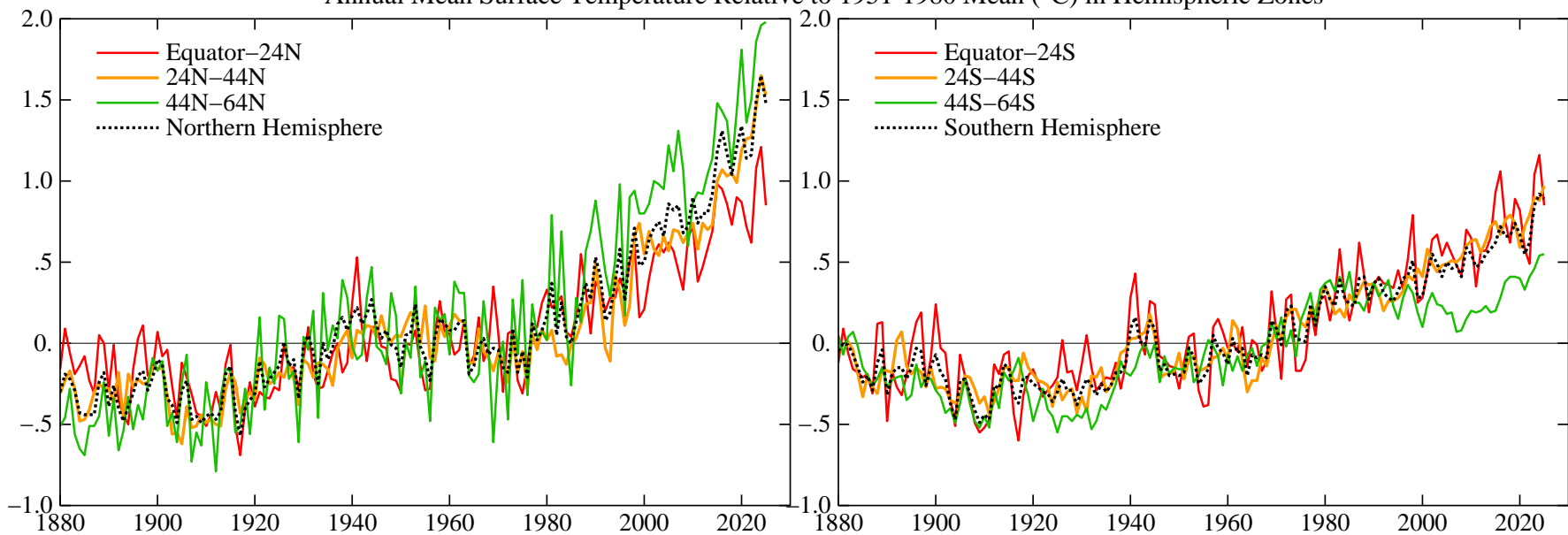
Annual Mean Surface Temperature Relative to 1951-1980 Mean (°C) in Hemispheric Zones
