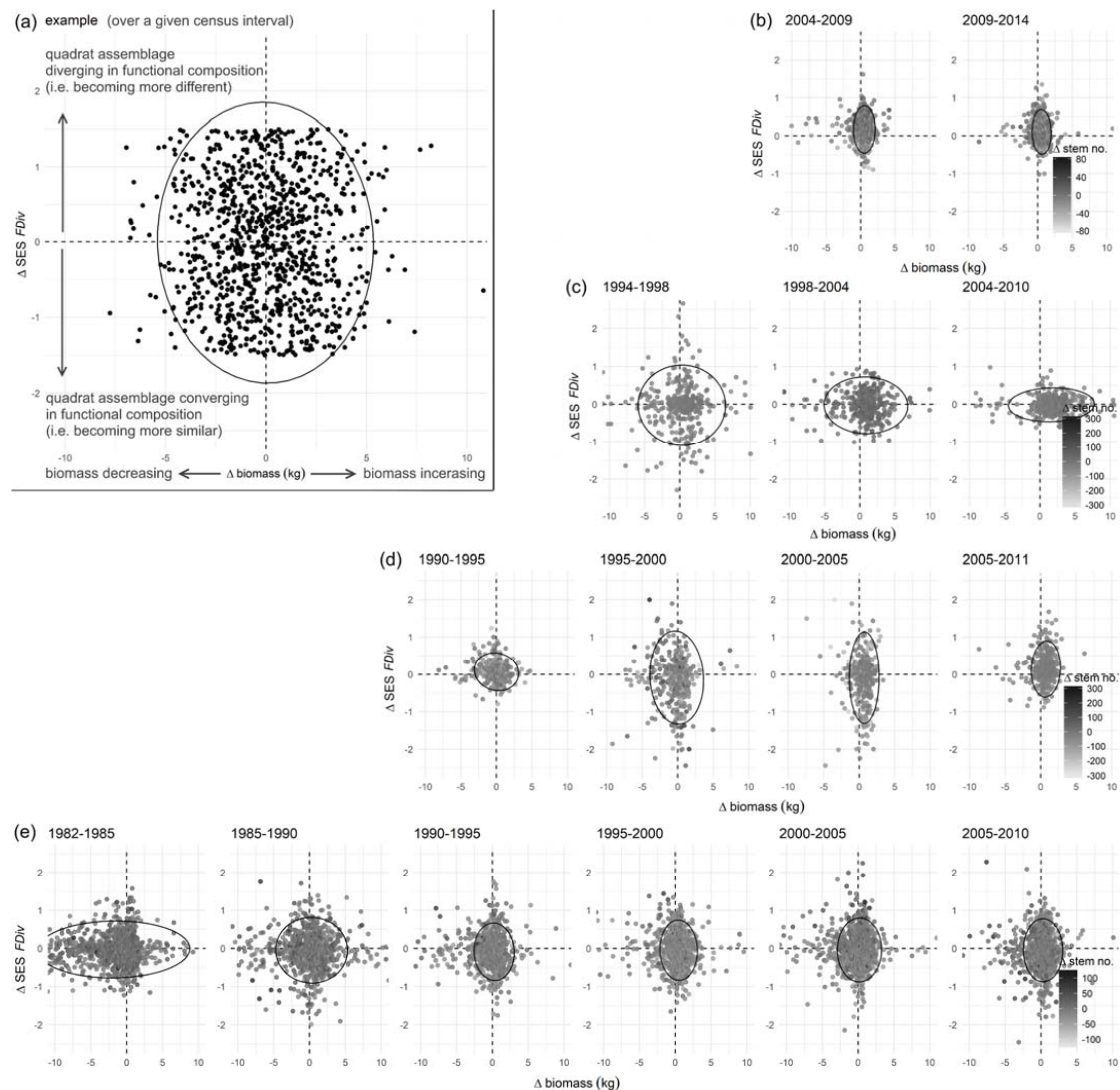
Figure 5. The change in quadrat biomass ( \Delta biomass) in kilograms plotted against the change in the standardized effect size of Functional Divergence ( \Delta SES FDiv ) of the quadrat species assemblage over 5-year census intervals for the 4 cyclonic storm-affected permanent forest dynamics FDPs: (b) Fushan, Taiwan; (c) Palanan, Philippines; (d) Luquillo, Puerto Rico; and (e) Barro Colorado Island (BCI), Panama. 95% Confidence ellipses shown. The example (a) shows a perfectly uniform relationship between \Delta biomass and \Delta SES FDiv . Ellipses wider than tall illustrate greater community change in biomass than functional divergence over a given ca. 5-year census interval, while ellipses taller than wide illustrate the opposite. Note that four major cyclonic storms have affected the Fushan plot (b) in two census intervals—Typhoons Area (2004), Jangmi (2008), Sinlaku (2008), and Soulik (2013); Three storms have affected the Palanan plot (c) over three census intervals—Typhoons Zeb (1998), Imbudo (2003), and Mitag (2007); And two major storms have occurred over four census intervals for the Luquillo plot (d)—Hurricanes Hugo (1989) and Georges (1998).
