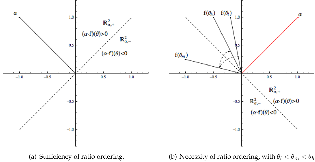
Figure 3: Ratio ordering and single crossing of all linear combinations.
