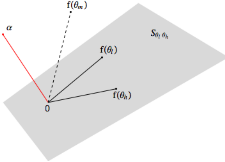
Figure 4: The necessity of linear dependence in Proposition 2 .
