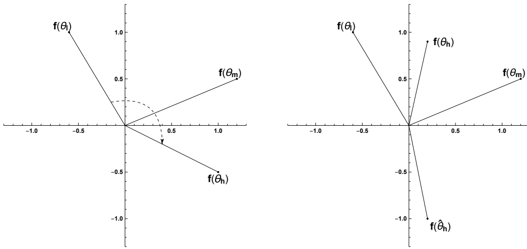
(a) Condition (6) holds for \theta_l < \theta_m < \theta_h .
