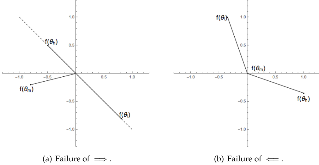
Figure 5: f_1 and f_2 are not ratio ordered because Condition (7) fails for \theta_l < \theta_m < \theta_h .
