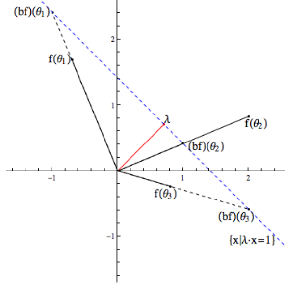
Figure 6: A geometric intuition for sufficiency of (iii) in Proposition 5.
