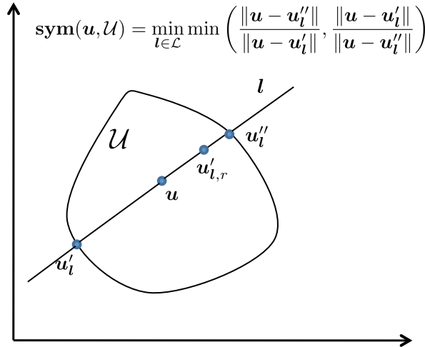
Figure 3: Geometric illustration of \text{sym}(\mathbf{u}, \mathcal{U}) .
