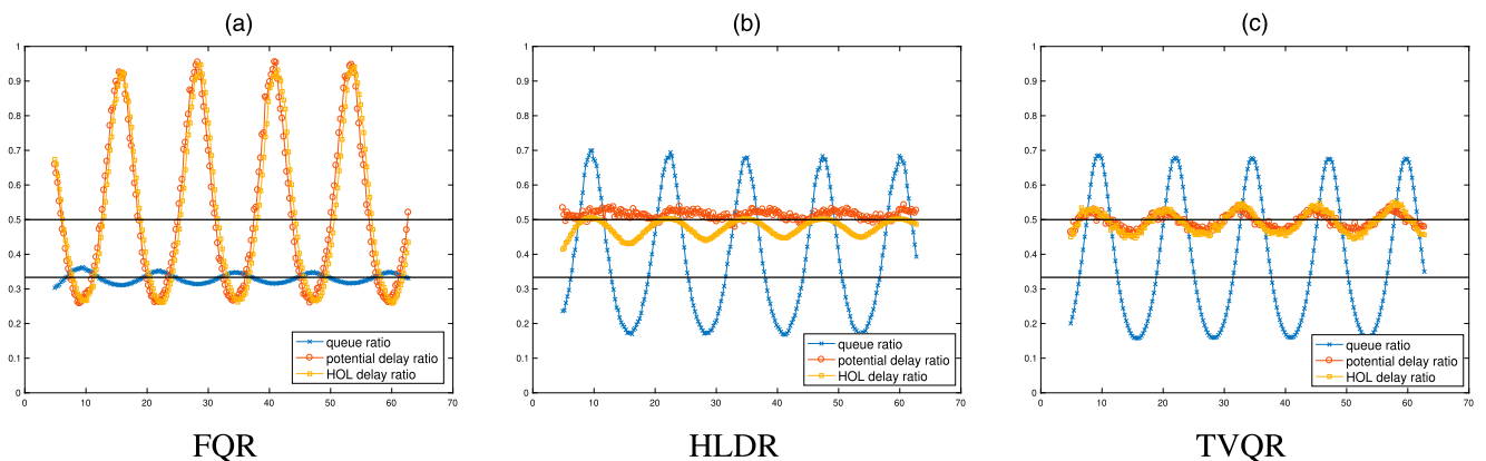
Figure 2. Queue and Delay Ratios for a Two-Class M_t/M/s_t Queue with Arrival Rate Functions \lambda_1(t) = 60 - 20 \sin(t/2) , \lambda_2 = 90 + 30 \sin(t/2) , Common Service Rate \mu = 1 , Without Abandonment ( \theta_1 = \theta_2 = 0 ), and \tilde{c} = 0.25
