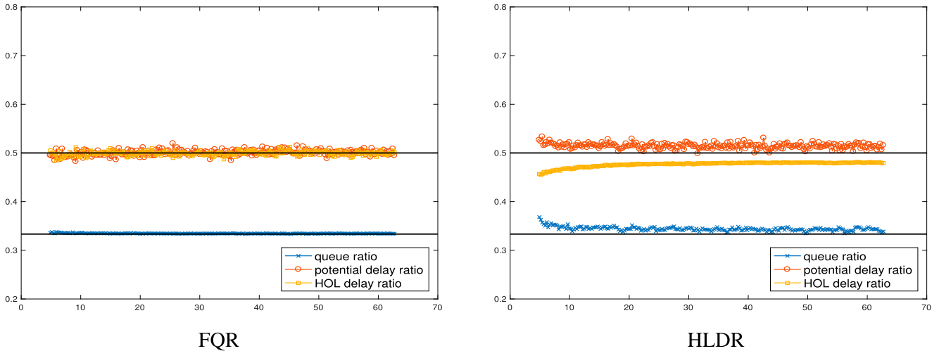
Figure 1. Queue and Delay Ratios for a Two-Class Stationary M/M/s Queue with Arrival Rate Functions \lambda_1 = 60, \lambda_2 = 90 , Common Service Rate \mu = 1 , Without Abandonment ( \theta_1 = \theta_2 = 0 ), and \tilde{c} = 0.25
