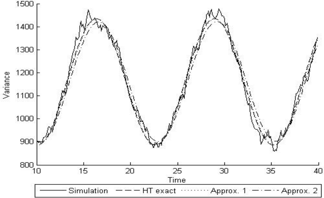
Figure 1: Comparison of simulated variance and its approximation functions in the M_t^B/M^D/\infty queue with B as a mixture, B = 1 w.p. 8/9 and B \sim Geom(0.1) w.p. 1/9 . m_S = 1 and \rho = 0.25 . \lambda_B(t) = 80 + 20 \sin(0.5t) .
