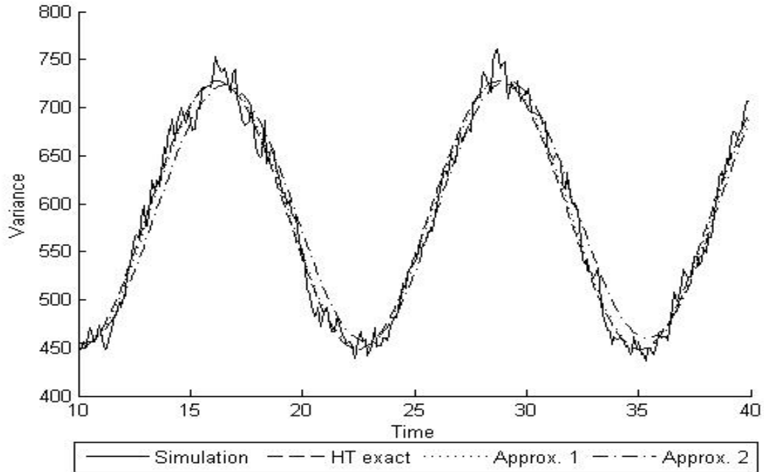
Figure 2: Comparison of simulated variance and its approximation functions in the M_t^B/H_2^D/\infty queue with B as a mixture, B = 1 w.p. 8/9 and B \sim \text{Geom}(0.1) w.p. 1/9 and H_2 service times with parameters \alpha_1 = \alpha_2 = 0.5, \mu_1 = 1, \mu_2 = 10, \rho_1 = 0.1, \rho_2 = 0.5 , so that m_S = 0.55 and \rho = 0.360 . \lambda_B(t) = 80 + 20 \sin(0.5t) .
