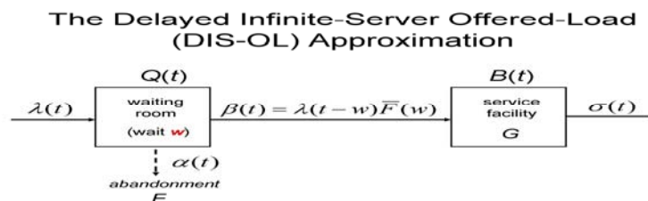
Figure 3. The delayed infinite-server offered-load (DIS-OL) approximation for the M_t / GI / s_t + GI queueing model. The contents Q(t) and B(t) are independent Poisson random variables for each t ; the three flows are Poisson processes.
