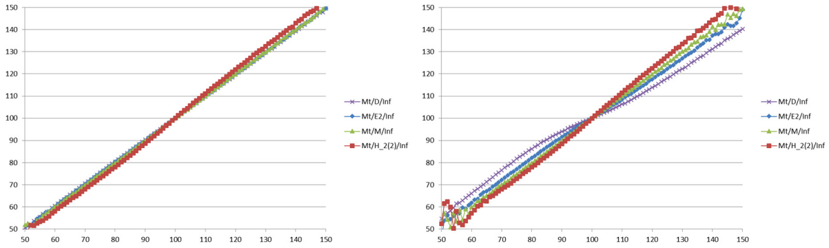
Figure 7. Estimated death rates for the M_t/GI/\infty model with the sinusoidal arrival rate function in (8) having parameters \bar{\lambda} = 100 and \beta = 10/35 and four different service-time distributions for \gamma = 1/2 (left) and \gamma = 2 (right). [Color figure can be viewed in the online issue, which is available at wileyonlinelibrary.com .]
