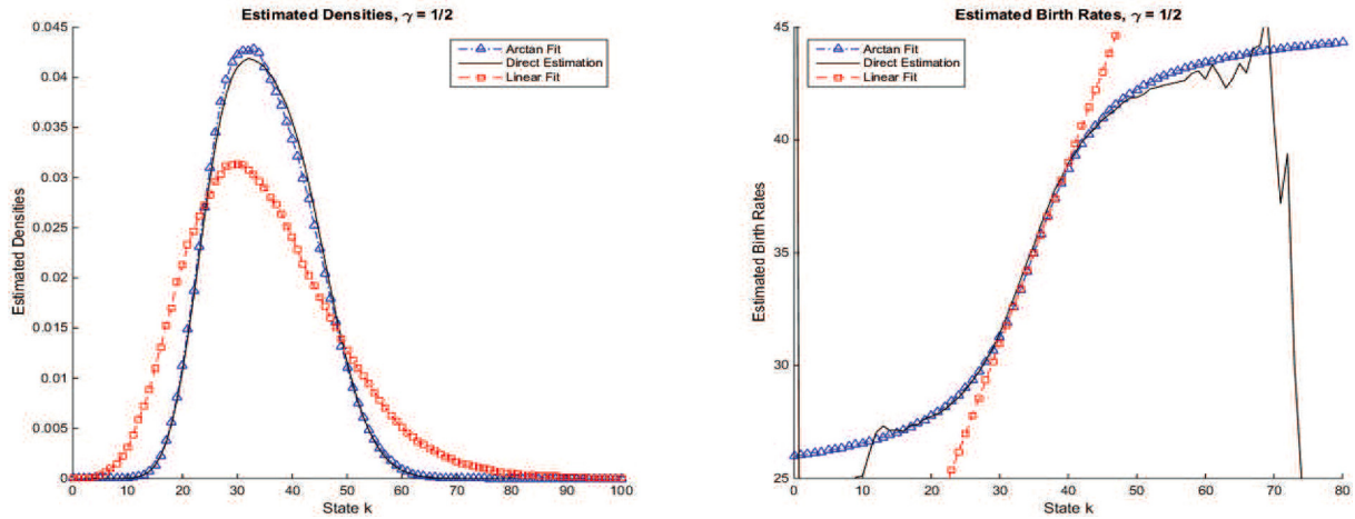
Figure 15. Fitted mass function (left) and birth rates (right) for the M_1/M/\infty model with the sinusoidal arrival rate function in (8) having parameters \bar{\lambda} = 35 , \beta\bar{\lambda} = 10 and \gamma = 0.5 . [Color figure can be viewed in the online issue, which is available at wileyonlinelibrary.com .]
