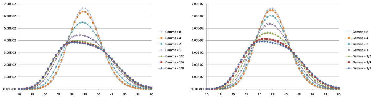
Figure 6. Fitted steady-state mass functions for the M_1/H_2/\infty model (left) and the M_1/E_2/\infty model (right) for with the sinusoidal arrival rate function in (8) having parameters \bar{\lambda} = 35 and \beta\bar{\lambda} = 10 and 7 values of \gamma ranging from 1/8 to 8 . [Color figure can be viewed in the online issue, which is available at wileyonlinelibrary.com .]
