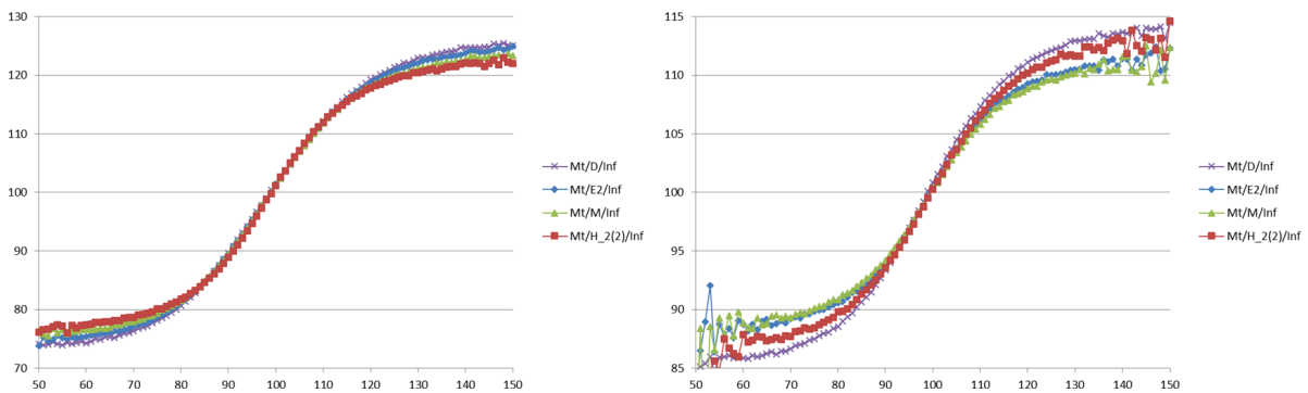
Figure 8. Estimated birth rates for the M_t/GI/\infty model with the sinusoidal arrival rate function in (8) having parameters \bar{\lambda} = 100 and \beta = 10/35 and four different service-time distributions for \gamma = 1/2 (left) and \gamma = 2 (right). [Color figure can be viewed in the online issue, which is available at wileyonlinelibrary.com .]
