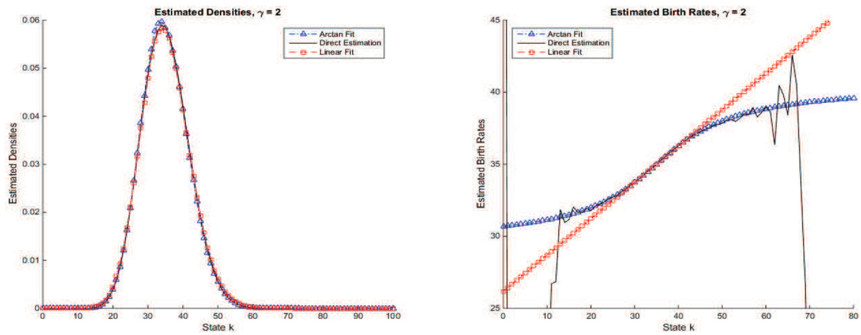
Figure 16. Fitted mass function (left) and fitted birth rates (right) for the M_1/M/\infty model with the sinusoidal arrival rate function in (8) having parameters \bar{\lambda} = 35 , \beta\bar{\lambda} = 10 and \gamma = 2.0 . [Color figure can be viewed in the online issue, which is available at wileyonlinelibrary.com .]
