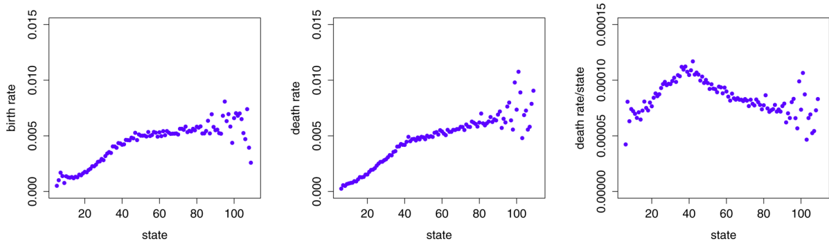
Figure 23. The fitted state-dependent birth rate \bar{\lambda}_k (left), death rate \bar{\mu}_k (center) and death rate divided by the state, \bar{\mu}_k/k (right) obtained from arrival and departure data in an Israeli emergency department over 25 weeks, taken from [36]. [Color figure can be viewed in the online issue, which is available at wileyonlinelibrary.com .]
