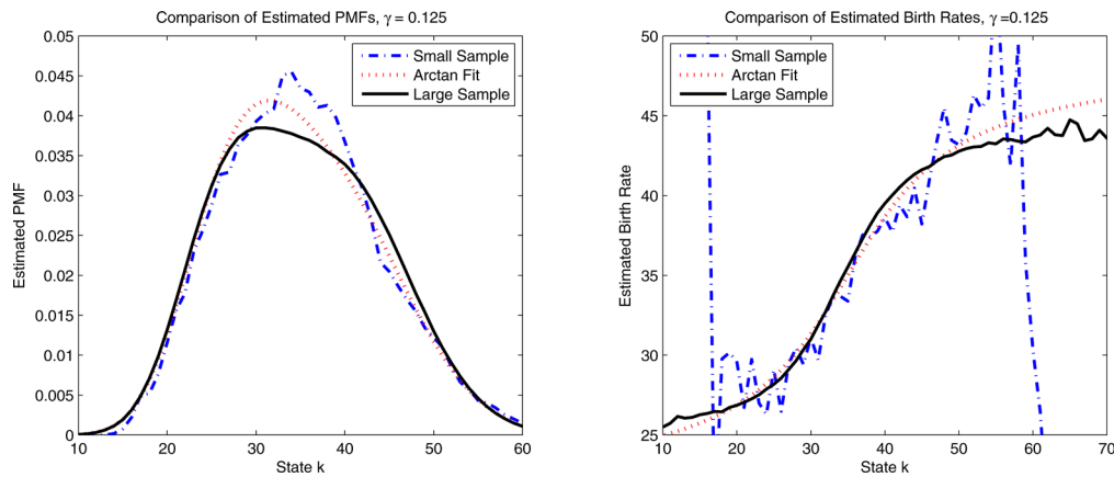
Figure 17. A comparison of the arctan BD fit to a small-sample direct fit of the steady-state probability mass function (left) and birth rates (right) for the M_1/M/\infty model with the sinusoidal arrival rate function in (8) having parameters \bar{\lambda} = 35 , \beta\bar{\lambda} = 10 , and \gamma = 0.125 . Data are collected from 10 cycles as indicated. The previous large-sample fit is used to represent the “true value.” [Color figure can be viewed in the online issue, which is available at wileyonlinelibrary.com .]
