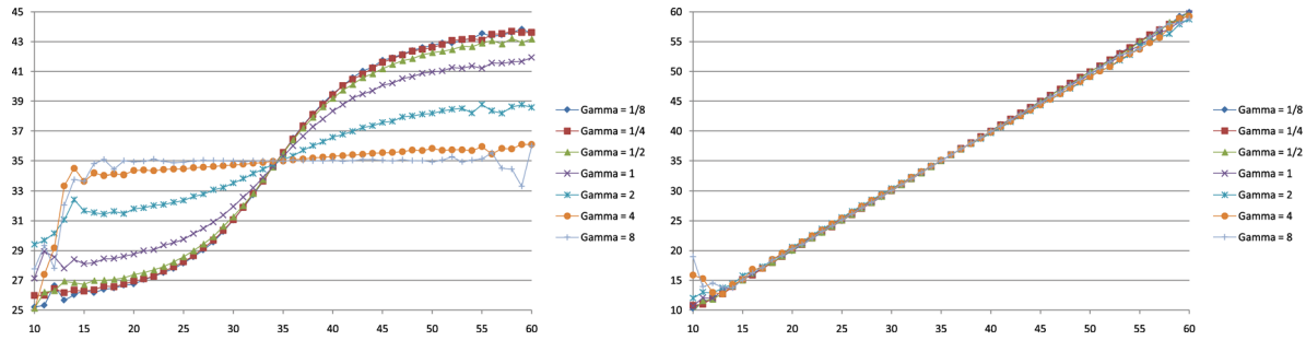
Figure 5. Fitted birth rates (left) and fitted death rates (right) for the M_1/E_2/\infty model with the sinusoidal arrival rate function in (8) having parameters \bar{\lambda} = 35 and \beta\bar{\lambda} = 10 and 7 values of \gamma ranging from 1/8 to 8 . [Color figure can be viewed in the online issue, which is available at wileyonlinelibrary.com .]
