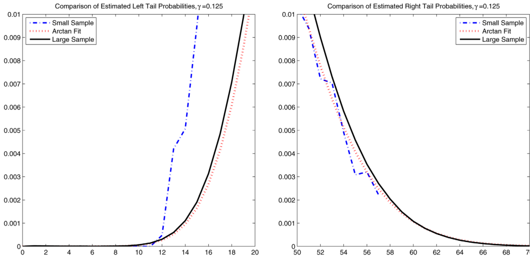
Figure 20. A comparison of the arctan BD fit to a small-sample direct fit of the steady-state tail probabilities (left) and (right) with data from one cycle instead of ten cycles. [Color figure can be viewed in the online issue, which is available at wileyonlinelibrary.com .]
