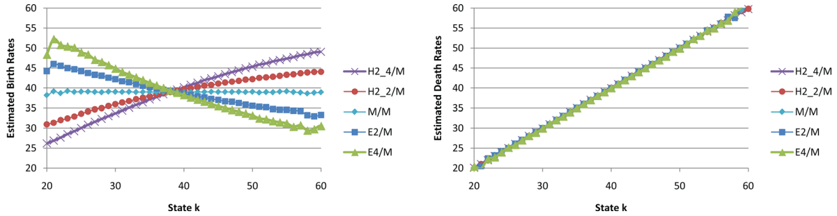
Figure 21. Fitted birth rates and death rates for five G/M/\infty models with \lambda = 39 and \mu = 1 . [Color figure can be viewed in the online issue, which is available at wileyonlinelibrary.com .]
