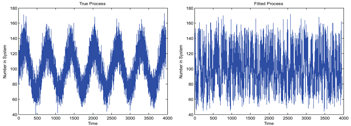
Figure 10. Sample paths of the number in system for the original process (left) and the fitted BD process (right) for the M_t/M/\infty queue with the sinusoidal arrival rate function in (8) having parameters \bar{\lambda} = 100 and \beta = 10/35 and \gamma = 0.01 . [Color figure can be viewed in the online issue, which is available at wileyonlinelibrary.com .]
