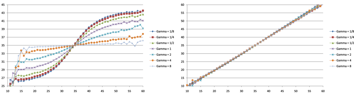
Figure 4. Fitted birth rates (left) and fitted death rates (right) for the M_t/H_2/\infty model with the sinusoidal arrival rate function in (8) having parameters \bar{\lambda} = 35 and \beta\bar{\lambda} = 10 and 7 values of \gamma ranging from 1/8 to 8 . (The service SCV is c^2 = 2 ). [Color figure can be viewed in the online issue, which is available at wileyonlinelibrary.com .]
