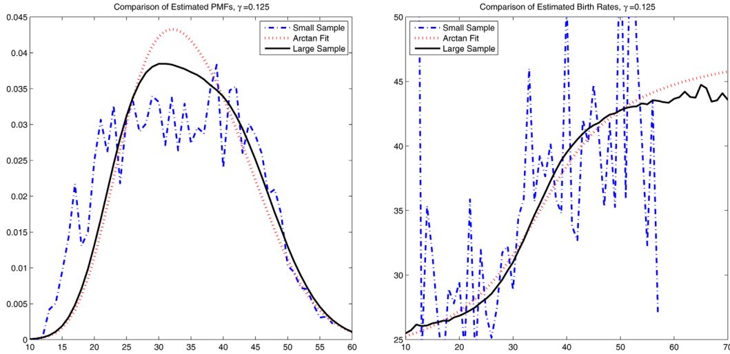
Figure 19. A repeat of the experiment in 17 with data from one cycle instead of 10 cycles. Estimates are shown of the steady-state probability mass function (left) and birth rates (right). [Color figure can be viewed in the online issue, which is available at wileyonlinelibrary.com .]
