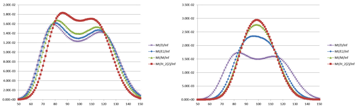
Figure 9. Estimated steady-state PMF's for the M_t/GI/\infty model with the sinusoidal arrival rate function in (8) having parameters \bar{\lambda} = 100 and \beta = 10/35 and four different service-time distributions for \gamma = 1/2 (left) and \gamma = 2 (right). [Color figure can be viewed in the online issue, which is available at wileyonlinelibrary.com .]
