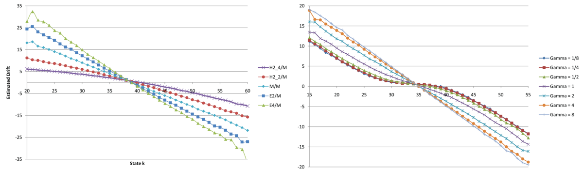
Figure 22. The estimated drift functions (birth rates minus death rates) in (55) for the G/M/\infty model in Figure 21 (left) and the M_t/M/\infty model in Figure 1 (right). [Color figure can be viewed in the online issue, which is available at wileyonlinelibrary.com .]
