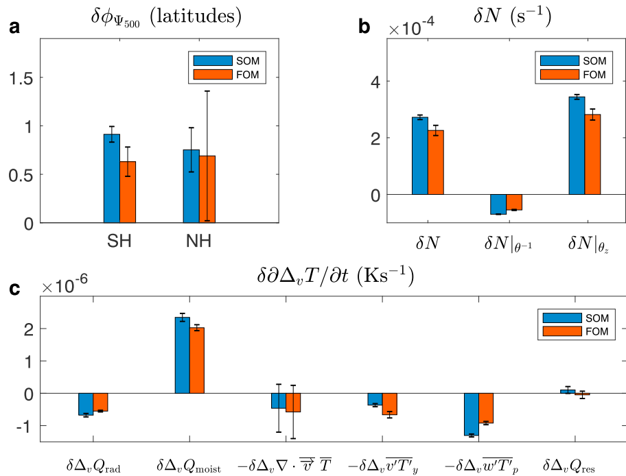
Figure 2. (a) The poleward shift of the Hadley cell edge ( \delta\phi_{\Psi_{500}} , degrees latitudes, section 2) in the SH and NH. (b) SH subtropical static stability response ( \delta N , s^{-1} ), separated to changes in mean potential temperature ( \delta N|_{\theta-1} , s^{-1} ) and to changes in the temperature lapse rate ( \delta N|_{\theta_z} , s^{-1} ). (c) The response of the SH subtropical vertical difference temperature tendency equation ( \delta \frac{\partial \Delta_v T}{\partial t} , K/s , equation (3)); radiation ( \delta\Delta_v Q_{rad} ), convection ( \delta\Delta_v Q_{moist} ), mean temperature flux convergence ( -\delta\Delta_v \nabla \cdot \bar{v}T ), meridional ( -\delta\Delta_v \bar{v}'T'_y ) and vertical ( -\delta\Delta_v \bar{w}'T'_p ) eddy temperature flux convergence, and adiabatic and vertical diffusion ( \delta\Delta_v Q_{res} ). Blue and red bars show the SOM and FOM responses, respectively. Vertical error bars represent the 95% confidence interval over the analysis period. SH = Southern Hemisphere; NH = Northern Hemisphere; SOM = slab ocean model; FOM = fully coupled ocean-atmosphere model.
