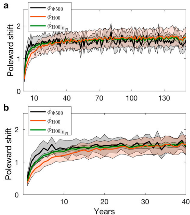
FIG. 6. (a) The annual and zonal multimodel-mean evolution relative to preindustrial values of the Hadley cell edge \phi_{\Psi 500} ( ^{\circ} lat; black line), the Hadley cell edge based on Held (2000) scaling \phi_{H00} [ ^{\circ} lat; red line; Eq. (2), using constant of proportionality of 0.8], and the Hadley cell edge based on Held (2000) scaling but with keeping tropopause height as in preindustrial values \phi_{H00|HPI} ( ^{\circ} lat; green line, using constant of proportionality of 2). (b) As in (a), but only focusing on the first 40 years. The shading in both panels represents the 95% confidence interval calculated via the Student's t test across all models.
