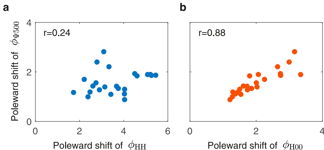
FIG. 5. The statistically steady-state Hadley cell edge \phi_{\Psi 500} ( ^{\circ} lat) poleward shift, relative to preindustrial values, as a function of the poleward shift of the Hadley cell edge ( ^{\circ} lat), based on (a) the Held and Hou (1980) scaling \phi_{HH} [Eq. (1)], and (b) the Held (2000) scaling \phi_{H00} [Eq. (2)]. Each dot in (a) and (b) represents one model simulation averaged over the last 50 years of simulation.
