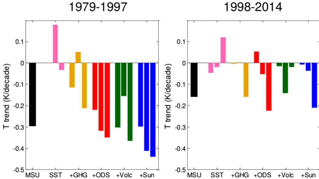
FIG. 3. Tropical T_{LS} trends for each model integration ( \text{K decade}^{-1} ), computed over the period (left) 1979–97 and (right) 1998–2014. Black bars: MSU observations; colored bars: the GEOS CCM integrations, forced as per the labels on the abscissa.
