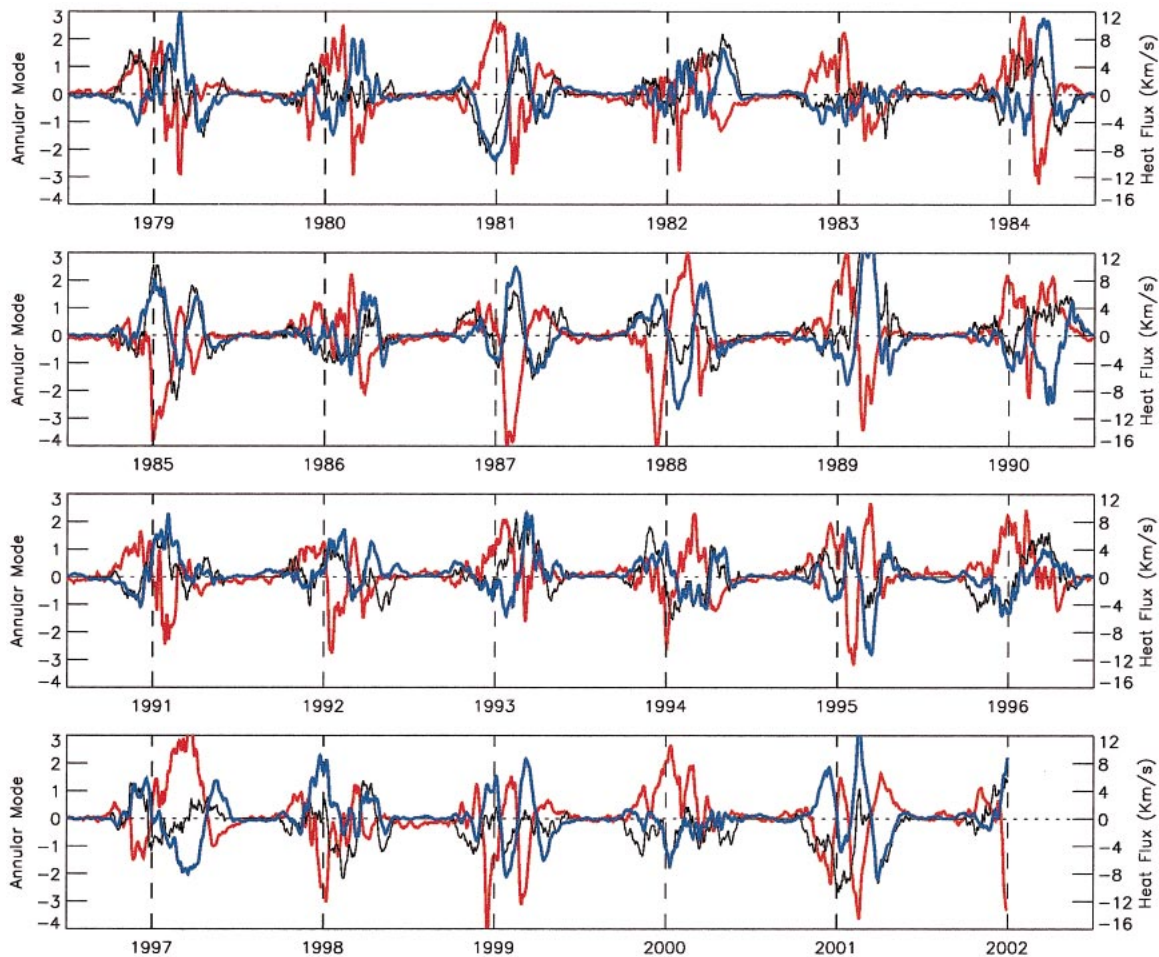
FIG. 2. Daily values of the NAM index at 10 hPa (red) and 40-day averaged heat flux anomalies at 100 (blue) and 300 hPa (black), for 1 Jul 1978–31 Dec 2002. Heat fluxes are averaged over 40 days up to the given day. The heat flux at 300 hPa has been multiplied by a factor of 2. The dashed vertical lines mark 1 Jan of each year.
