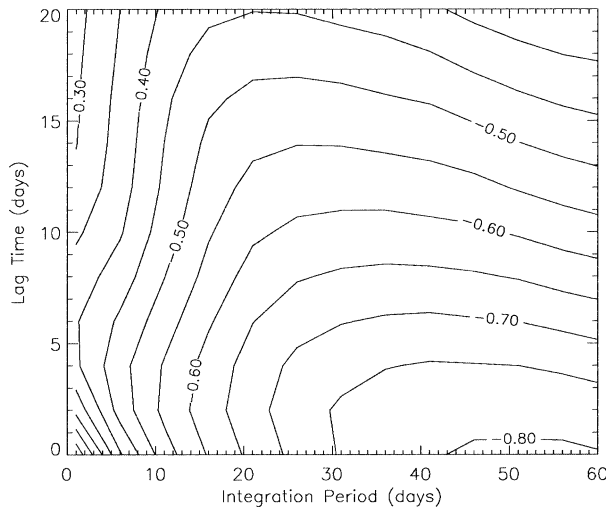
FIG. 3. The correlation coefficient between the NAM index at 10 hPa and the averaged heat flux at 100 hPa, as a function of the integration period for the heat flux and time lag between the end of that integration period and the time of the NAM index. The contour interval is 0.05. Data for all winters (Dec–Feb) from 1958 to 2001 are used to compute these correlations.
