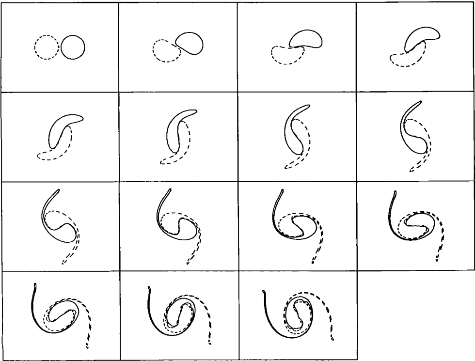
FIGURE 6. Alignment for d_c = 2.2 and \gamma = 5.0 . Time advances to the right and downwards. The frames are shown at t = 0, 0.5, 1.0, 1.5, \dots . The two vortices are located in different layers.
