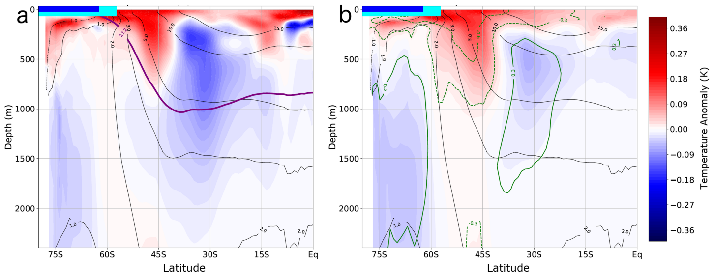
Figure 2. Ocean temperature anomaly (colors; K) when Antarctic SIA is low in the CESM1 LE Control: (a) at Year 1189 (with the 27.2\sigma isopycnal surface; thick purple contour) and (b) regressed on the Antarctic SIA, shown at two standard deviations below the climatological mean (the correlations for the regression are shown as green contours at r = [-0.6, -0.3, 0.3] ). Annual mean temperatures (black contours) are shown in both panels. Sea ice extent (the mean latitude of the 0.15 ice fraction contour) in DJF (dark blue) and JJA (cyan) is shown (a) at Year 1189 in the CESM1 LE Control and (b) regressed on SIA in the CESM1 LE Control at two standard deviations below the climatological mean.
