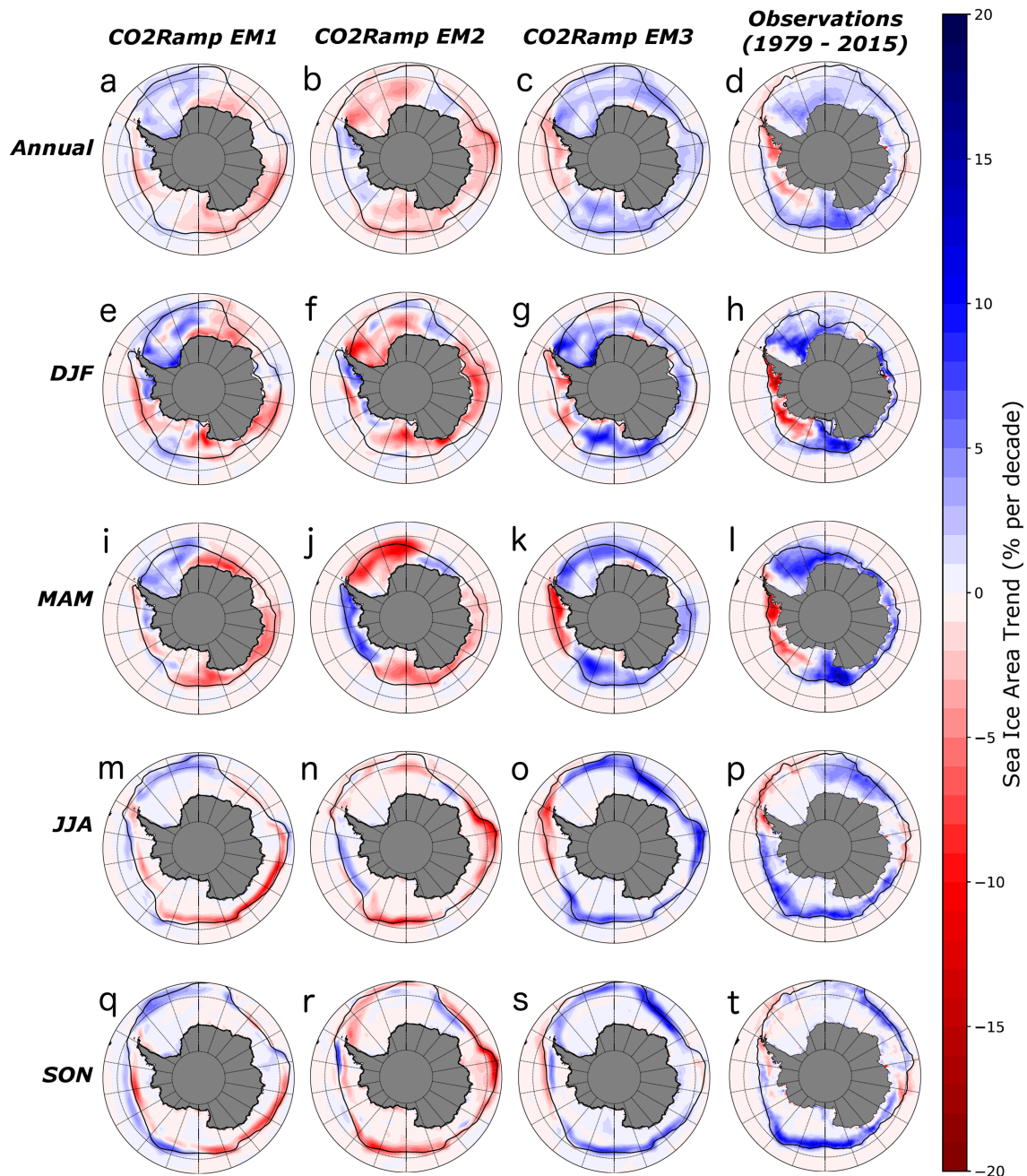
Figure 4. Regional trends in Antarctic SIA (% per decade) in the three CESM1 CO2Ramp ensemble members (Years 0 to 26) and in observations (1979 to 2015): (a–d) in the annual mean, (e–h) December–January–February (DJF), (i–l) March–April–May (MAM), (m–p) June–July–August (JJA), and (q–t) September–October–November (SON) for CO2Ramp ensemble member 1 (EM1; a, e, i, m, and q), CO2Ramp ensemble member 2 (EM2; b, f, j, n, and r), CO2Ramp ensemble member 3 (EM3; c, g, k, o, and s), and observations (d, h, l, p, and t). In all panels, the 15% sea ice fraction contour is indicated (black line).
