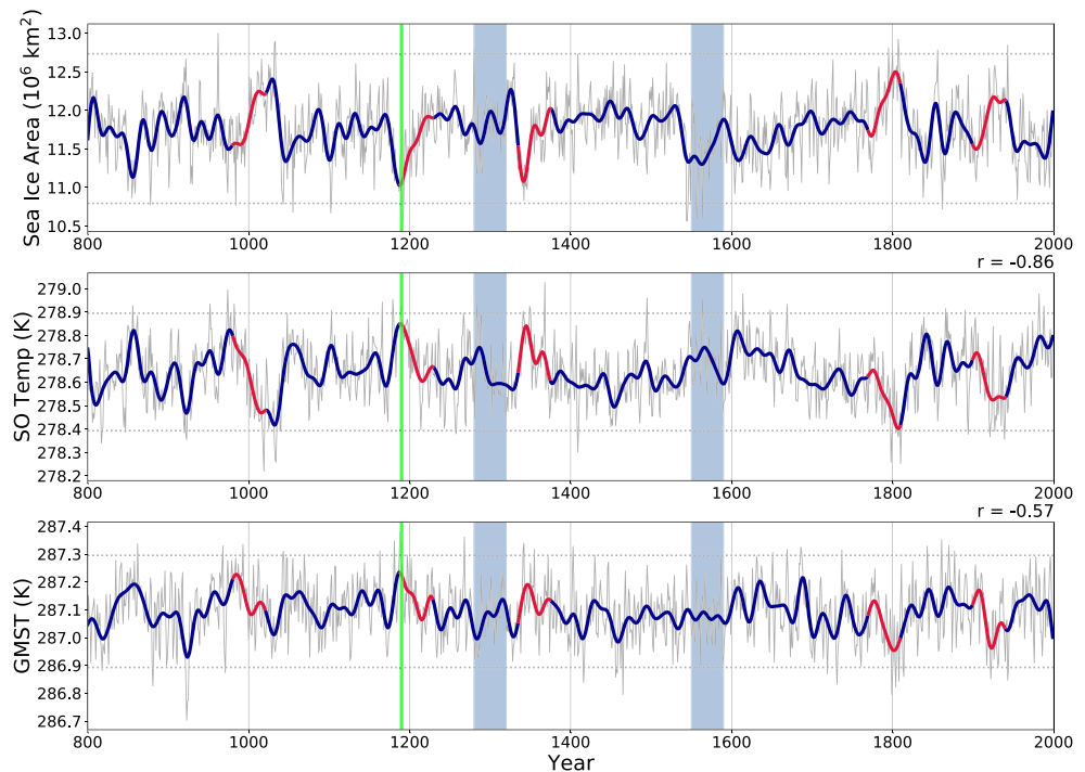
Figure 1. Internal variability over 1,200 years of the CESM1 Large Ensemble Control (LEControl): (a) annual mean Antarctic SIA ( 10^6 km 2 ); (b) annual mean Southern Ocean SST (from 45° S to 60° S; K); and (c) annual global mean surface temperature (GMST; K). Thin gray lines show the annual mean time series, with 2 standard deviations above and below the mean indicated (dotted gray). Thick lines show the 10-year low-pass filtered time series (filtered using a ten-year Lanczos filter with 11 weights; see Duchon, 1979), with five 40-year time periods over which Antarctic SIA expands at a rate greater than that in observations (1979–2015) drawn in red. Highlighted blue areas indicate 30-year periods during which Antarctic SIA and Southern Ocean SSTs trends are in the same sense (i.e., increasing SIA and decreasing SSTs), but trends in GMST are in the opposite sense (see text). The year from which CO2Ramp ensemble members are branched, 1190, is indicated in all panels (green vertical line).
