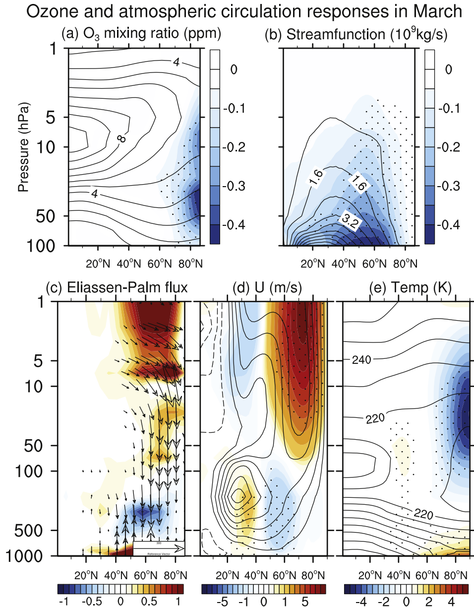
Figure 3. Distributions of March zonally averaged ozone and atmospheric circulation as a function of pressure and latitude for the control run climatology (contours) and the response to Arctic sea ice loss (shading; stippling indicates the 95% significance level). (a) Ozone mixing ratio (ppm), (b) Brewer–Dobson circulation ( 10^9 \text{ kg s}^{-1} ), (c) Eliassen–Palm (E–P) flux vector and its divergence ( \text{m s}^{-1} \text{ day}^{-1} ; shading). Note that the climatological E–P fluxes and divergence fields are not shown. (d) Zonal wind ( \text{m s}^{-1} ), (e) Temperature (K). The contour intervals for ozone mixing ratio, Brewer–Dobson circulation, zonal wind, and temperature are 1 ppm, 8 \times 10^8 \text{ kg s}^{-1} , 5 \text{ m s}^{-1} , and 10 K, respectively. For better display, we plot only those E–P vectors whose vertical component exceeds 10 \text{ Pa m s}^{-2} in absolute value. Note that a nonlinear color scale is used for the zonal wind response (interval of 0.25 \text{ m s}^{-1} for absolute value less than 1 \text{ m s}^{-1} and interval of 1 \text{ m s}^{-1} for absolute value larger than 1 \text{ m s}^{-1} ).
