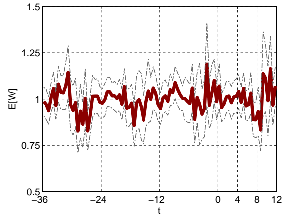
Figure 119: Average waiting time: QoS parameter \beta = 1 .
