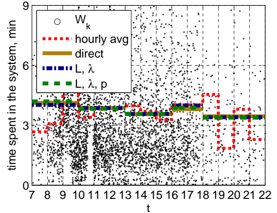
Figure 141: Scatter plot of the waiting times and its hourly averages, \bar{W}(t) , \bar{W}_{L,\lambda}(t) and \bar{W}_{L,\lambda,p}(t) of each hour in [7, 22] on May 16.
