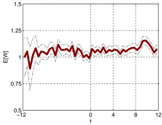
Figure 38: Average waiting time: QoS parameter \beta = 0 .
