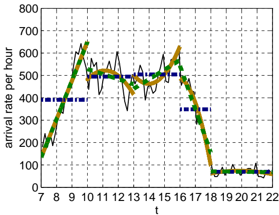
Figure 158: Arrival rate and its approximations by constant, linear and quadratic functions fitted to 5 intervals, [7, 10], [10, 13], [13, 16], [16, 18] and [18, 22], on May 30.
