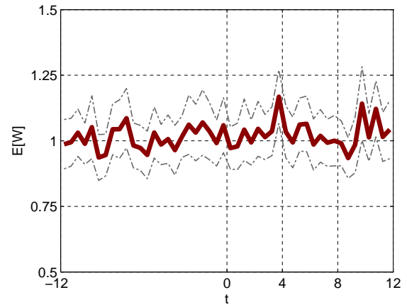
Figure 15: Average waiting time: QoS parameter \beta = 1 .
