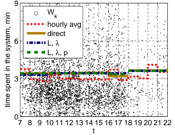
Figure 127: Scatter plot of the waiting times and its hourly averages, \bar{W}(t) , \bar{W}_{L,\lambda}(t) and \bar{W}_{L,\lambda,p}(t) of each hour in [7, 22] on May 2.
