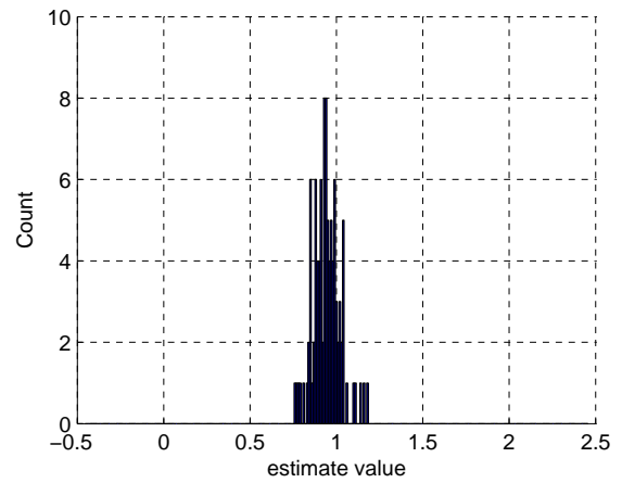
Figure 65: QoS \beta = 1 : Estimates on [0, 8]
