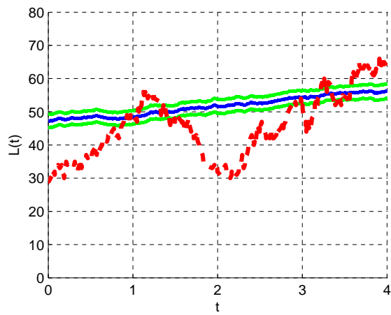
Figure 86: L(t) (dashed line) as well as average L(t) with associated 95% confidence interval based on 100 replications. \beta = 0 .
