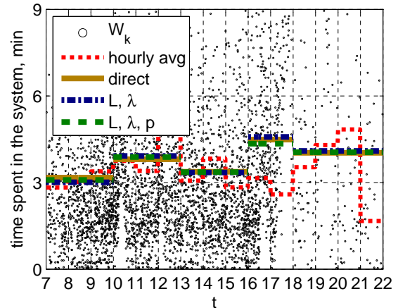
Figure 135: Scatter plot of the waiting times and its hourly averages, \bar{W}(t) , \bar{W}_{L,\lambda}(t) and \bar{W}_{L,\lambda,p}(t) of each hour in [7, 22] on May 11.
