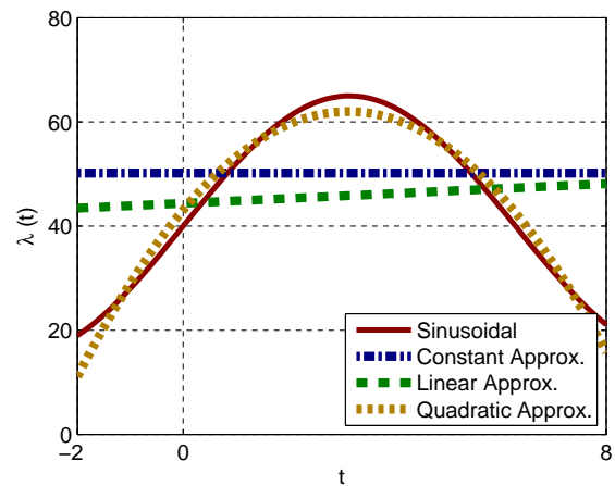
Figure 109: Fitting constant, linear and quadratic arrival rate functions over the intervals [-2, 8] to the arrival data for sinusoidal arrival process.
