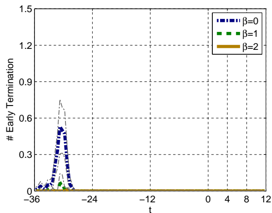
Figure 111: Number of early termination in each subinterval of length 0.5. H_2 service with sinusoidal arrival rate.
