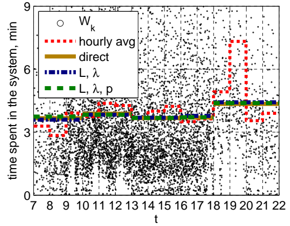
Figure 157: Scatter plot of the waiting times and its hourly averages, \bar{W}(t) , \bar{W}_{L,\lambda}(t) and \bar{W}_{L,\lambda,p}(t) of each hour in [7, 22] on May 29.
