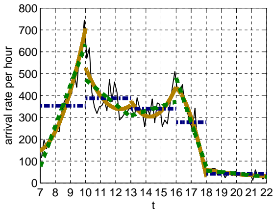
Figure 134: Arrival rate and its approximations by constant, linear and quadratic functions fitted to 5 intervals, [7, 10], [10, 13], [13, 16], [16, 18] and [18, 22], on May 11.
