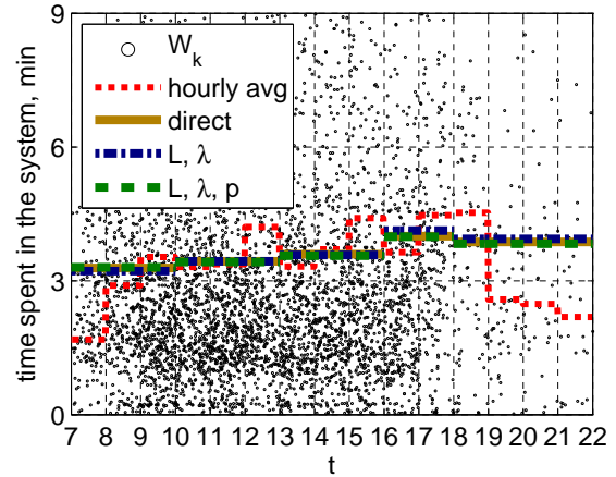
Figure 145: Scatter plot of the waiting times and its hourly averages, \bar{W}(t) , \bar{W}_{L,\lambda}(t) and \bar{W}_{L,\lambda,p}(t) of each hour in [7, 22] on May 18.
