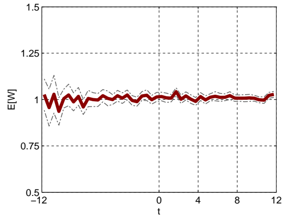
Figure 27: Average waiting time: QoS parameter \beta = 1 .
