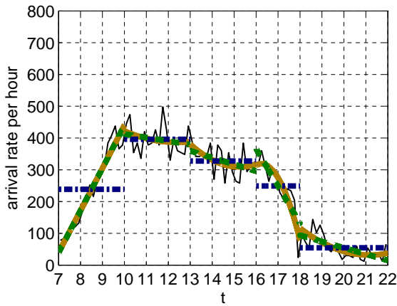
Figure 142: Arrival rate and its approximations by constant, linear and quadratic functions fitted to 5 intervals, [7, 10], [10, 13], [13, 16], [16, 18] and [18, 22], on May 17.
