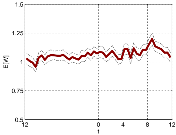
Figure 2: Average waiting time: QoS parameter \beta = 0 .
