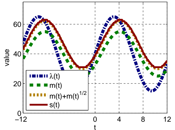
Figure 107: The sinusoidal arrival rate function, offered load function and staffing for H_2 service time distribution according to (8.1) with \beta = 1 based on starting empty in the distant past. These will be applied over the intervals [0, 4] and [0, 8] to the system starting empty at time -36 .
