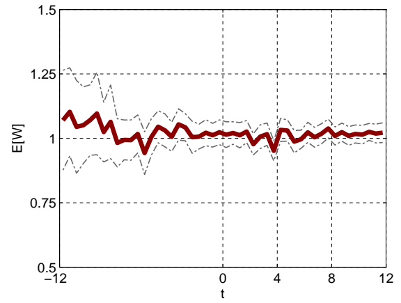
Figure 21: Average waiting time: QoS parameter \beta = 1 .
