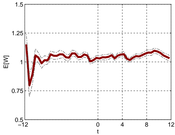
Figure 44: Average waiting time: QoS parameter \beta = 0 .
