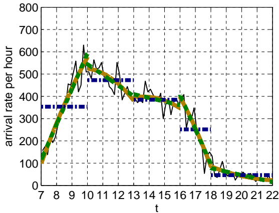
Figure 128: Arrival rate and its approximations by constant, linear and quadratic functions fitted to 5 intervals, [7, 10], [10, 13], [13, 16], [16, 18] and [18, 22], on May 4.
