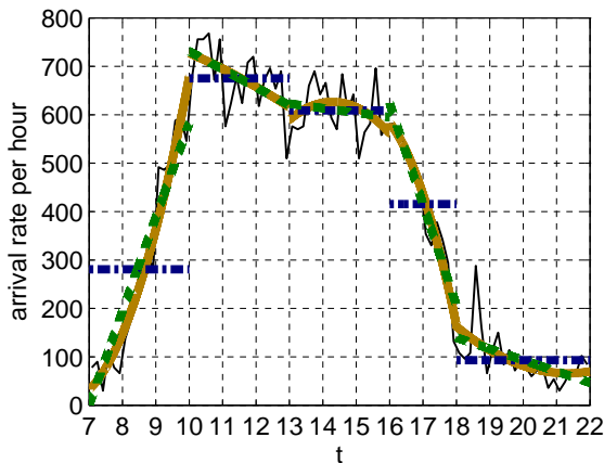
Figure 146: Arrival rate and its approximations by constant, linear and quadratic functions fitted to 5 intervals, [7, 10], [10, 13], [13, 16], [16, 18] and [18, 22], on May 21.
