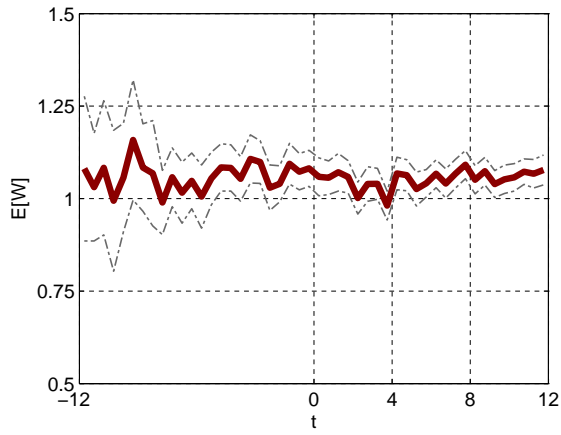
Figure 20: Average waiting time: QoS parameter \beta = 0 .
