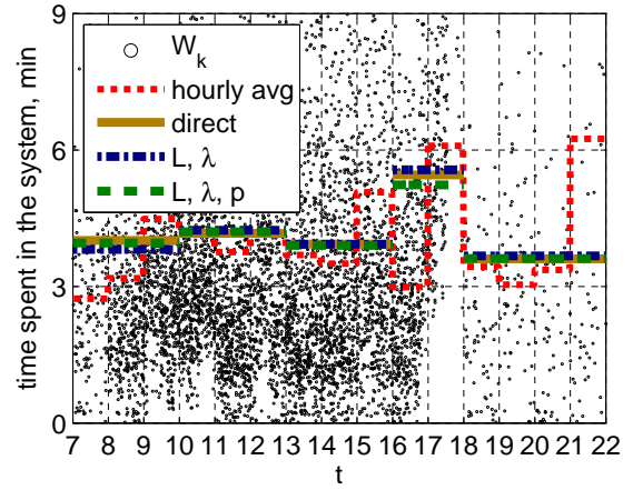
Figure 139: Scatter plot of the waiting times and its hourly averages, \bar{W}(t) , \bar{W}_{L,\lambda}(t) and \bar{W}_{L,\lambda,p}(t) of each hour in [7, 22] on May 15.
