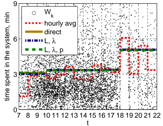
Figure 151: Scatter plot of the waiting times and its hourly averages, \bar{W}(t) , \bar{W}_{L,\lambda}(t) and \bar{W}_{L,\lambda,p}(t) of each hour in [7, 22] on May 23.
