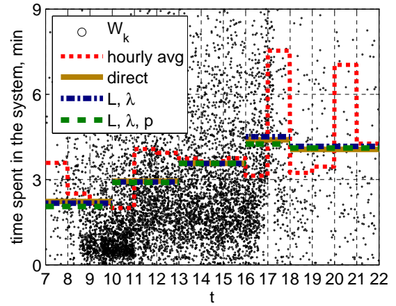
Figure 137: Scatter plot of the waiting times and its hourly averages, \bar{W}(t) , \bar{W}_{L,\lambda}(t) and \bar{W}_{L,\lambda,p}(t) of each hour in [7, 22] on May 14.
