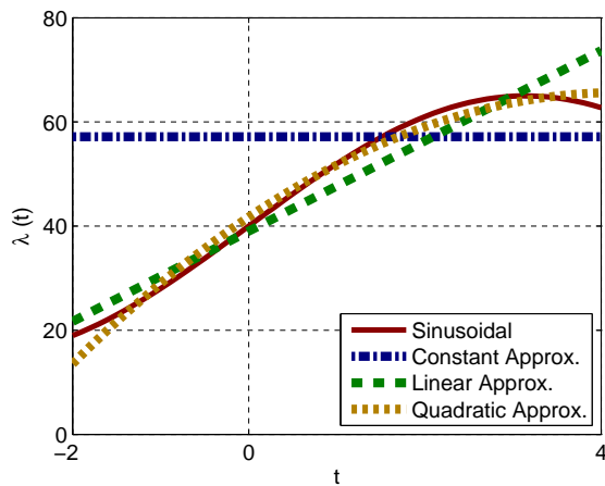
Figure 108: Fitting constant, linear and quadratic arrival rate functions over the intervals [-2, 4] to the arrival data for sinusoidal arrival process.
