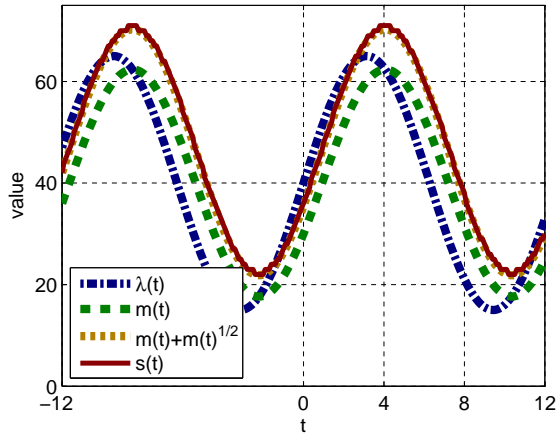
Figure 106: The sinusoidal arrival rate function, offered load function and staffing for exponential service time distribution according to (8.1) with \beta = 1 based on starting empty in the distant past. These will be applied over the intervals [0, 4] and [0, 8] to the system starting empty at time -36 .
