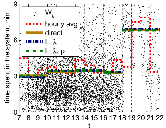
Figure 153: Scatter plot of the waiting times and its hourly averages, \bar{W}(t) , \bar{W}_{L,\lambda}(t) and \bar{W}_{L,\lambda,p}(t) of each hour in [7, 22] on May 24.
