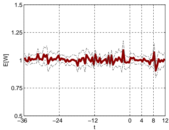
Figure 114: Average waiting time: QoS parameter \beta = 2 .
