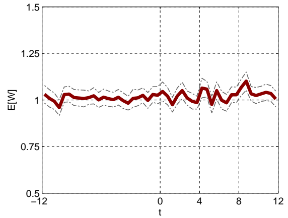
Figure 3: Average waiting time: QoS parameter \beta = 1 .
