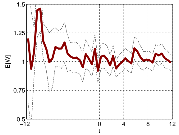
Figure 33: Average waiting time: QoS parameter \beta = 1 .
