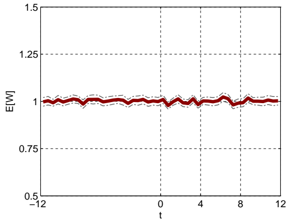
Figure 10: Average waiting time: QoS parameter \beta = 2 .
