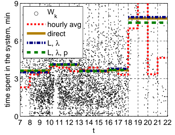
Figure 125: Scatter plot of the waiting times and its hourly averages, \bar{W}(t) , \bar{W}_{L,\lambda}(t) and \bar{W}_{L,\lambda,p}(t) of each hour in [7, 22] on May 1.
