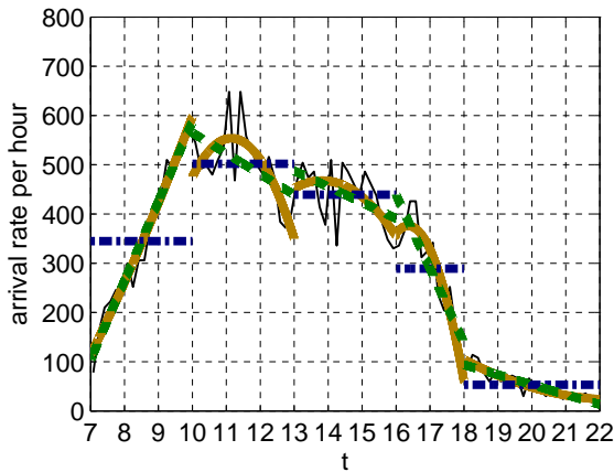
Figure 144: Arrival rate and its approximations by constant, linear and quadratic functions fitted to 5 intervals, [7, 10], [10, 13], [13, 16], [16, 18] and [18, 22], on May 18.
