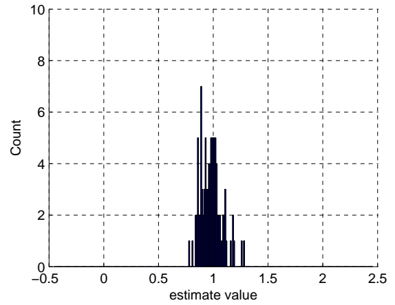
Figure 57: QoS \beta = 0 : Estimates on [0, 8]
