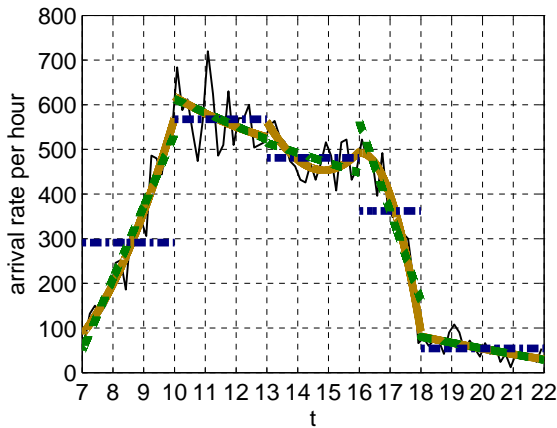
Figure 132: Arrival rate and its approximations by constant, linear and quadratic functions fitted to 5 intervals, [7, 10], [10, 13], [13, 16], [16, 18] and [18, 22], on May 8.
