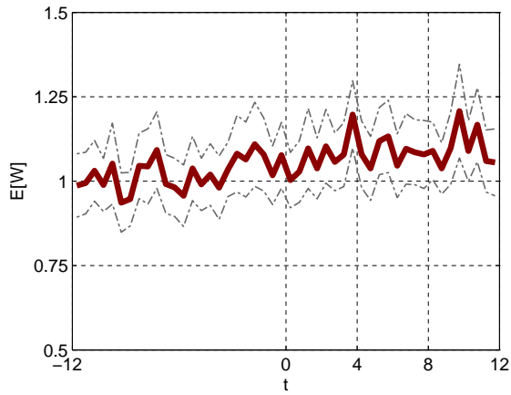
Figure 14: Average waiting time: QoS parameter \beta = 0 .
