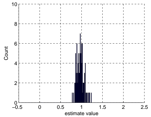
Figure 59: QoS \beta = 1 : Estimates on [0, 8]
