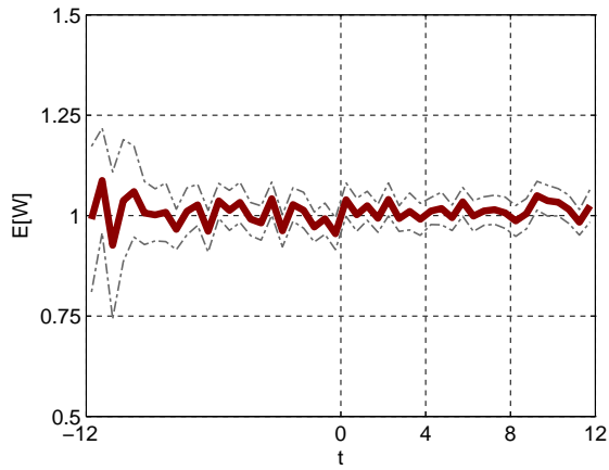
Figure 40: Average waiting time: QoS parameter \beta = 2 .
