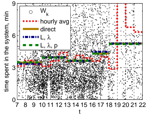
Figure 149: Scatter plot of the waiting times and its hourly averages, \bar{W}(t) , \bar{W}_{L,\lambda}(t) and \bar{W}_{L,\lambda,p}(t) of each hour in [7, 22] on May 22.
