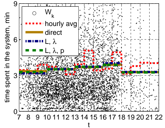
Figure 133: Scatter plot of the waiting times and its hourly averages, \bar{W}(t) , \bar{W}_{L,\lambda}(t) and \bar{W}_{L,\lambda,p}(t) of each hour in [7, 22] on May 8.
