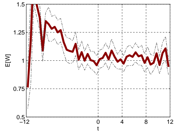
Figure 51: Average waiting time: QoS parameter \beta = 1 .
