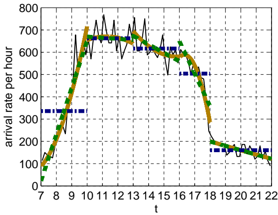
Figure 156: Arrival rate and its approximations by constant, linear and quadratic functions fitted to 5 intervals, [7, 10], [10, 13], [13, 16], [16, 18] and [18, 22], on May 29.
