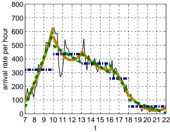
Figure 124: Arrival rate and its approximations by constant, linear and quadratic functions fitted to 5 intervals, [7, 10], [10, 13], [13, 16], [16, 18] and [18, 22], on May 1.
