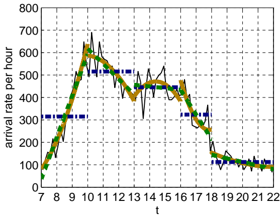
Figure 150: Arrival rate and its approximations by constant, linear and quadratic functions fitted to 5 intervals, [7, 10], [10, 13], [13, 16], [16, 18] and [18, 22], on May 23.
