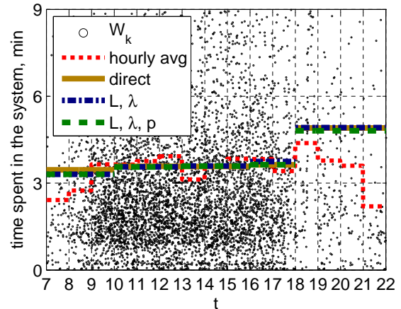
Figure 147: Scatter plot of the waiting times and its hourly averages, \bar{W}(t) , \bar{W}_{L,\lambda}(t) and \bar{W}_{L,\lambda,p}(t) of each hour in [7, 22] on May 21.
