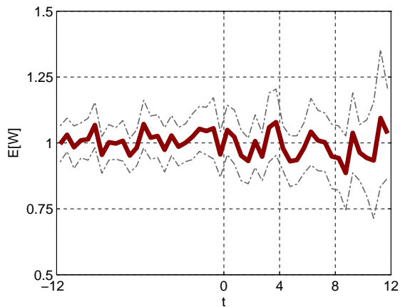
Figure 102: Average waiting time: QoS parameter \beta = 2 .
