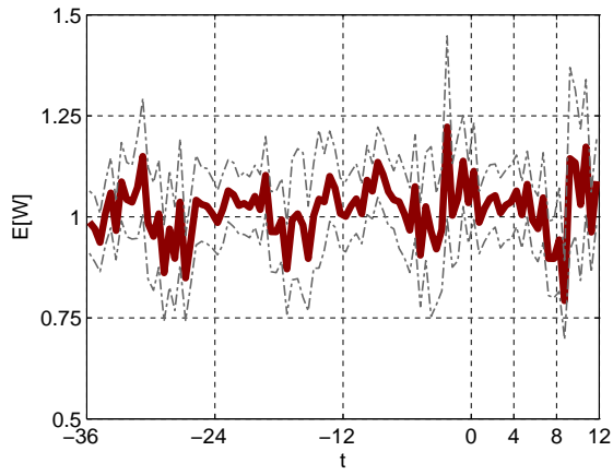
Figure 118: Average waiting time: QoS parameter \beta = 0 .
