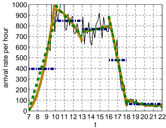
Figure 136: Arrival rate and its approximations by constant, linear and quadratic functions fitted to 5 intervals, [7, 10], [10, 13], [13, 16], [16, 18] and [18, 22], on May 14.
