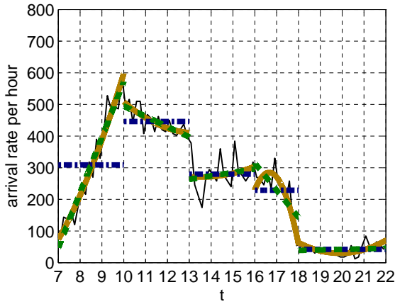
Figure 126: Arrival rate and its approximations by constant, linear and quadratic functions fitted to 5 intervals, [7, 10], [10, 13], [13, 16], [16, 18] and [18, 22], on May 2.
