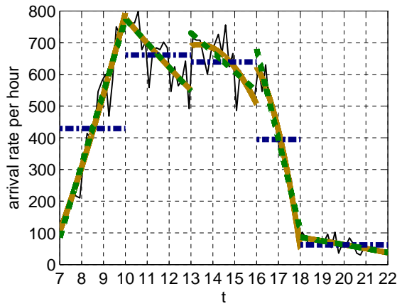
Figure 138: Arrival rate and its approximations by constant, linear and quadratic functions fitted to 5 intervals, [7, 10], [10, 13], [13, 16], [16, 18] and [18, 22], on May 15.
