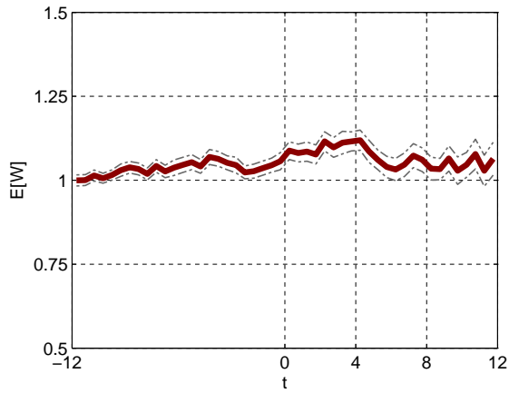
Figure 94: Average waiting time: QoS parameter \beta = 0 .
