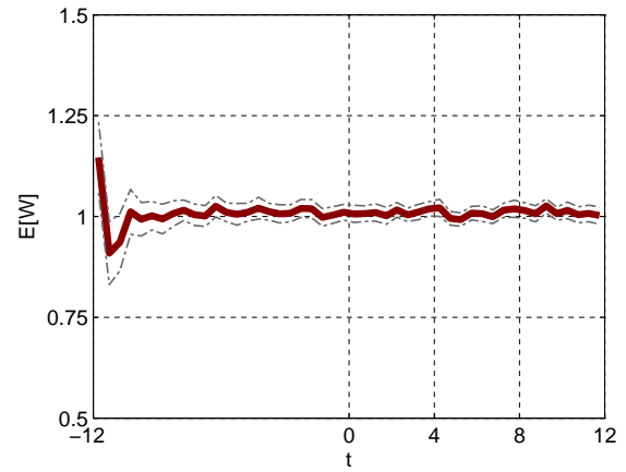
Figure 45: Average waiting time: QoS parameter \beta = 1 .
