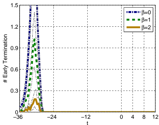
Figure 110: Number of early termination in each subinterval of length 0.5. M service with sinusoidal arrival rate.
