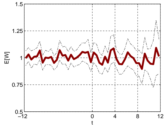
Figure 101: Average waiting time: QoS parameter \beta = 1 .
