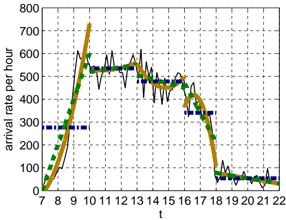
Figure 130: Arrival rate and its approximations by constant, linear and quadratic functions fitted to 5 intervals, [7, 10], [10, 13], [13, 16], [16, 18] and [18, 22], on May 7.
