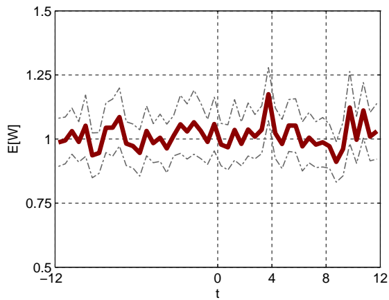
Figure 16: Average waiting time: QoS parameter \beta = 2 .
