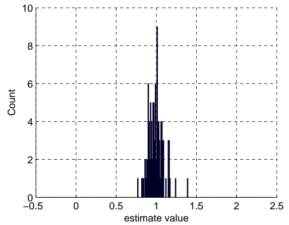
Figure 71: QoS \beta = 1 : Estimates on [0, 8]
