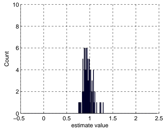
Figure 63: QoS \beta = 0 : Estimates on [0, 8]
