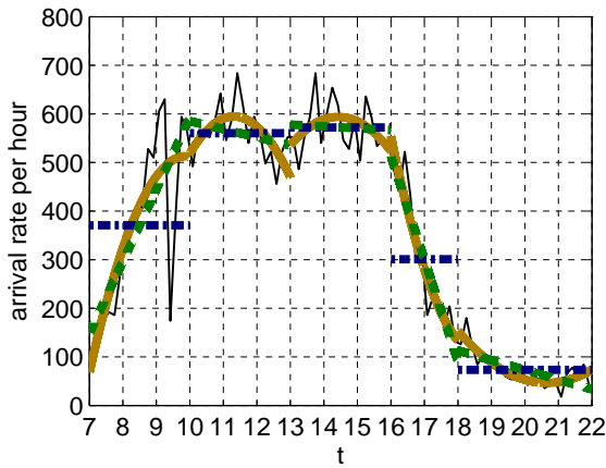
Figure 154: Arrival rate and its approximations by constant, linear and quadratic functions fitted to 5 intervals, [7, 10], [10, 13], [13, 16], [16, 18] and [18, 22], on May 25.
