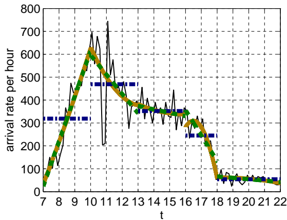
Figure 140: Arrival rate and its approximations by constant, linear and quadratic functions fitted to 5 intervals, [7, 10], [10, 13], [13, 16], [16, 18] and [18, 22], on May 16.
