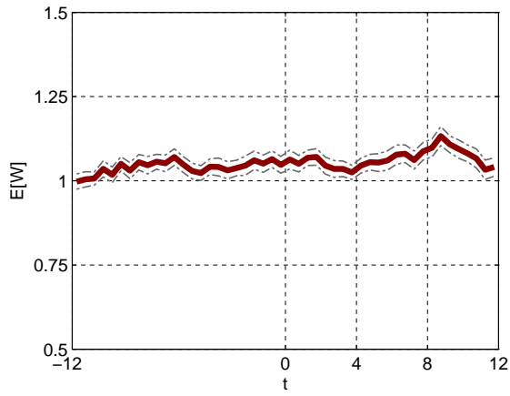
Figure 8: Average waiting time: QoS parameter \beta = 0 .
