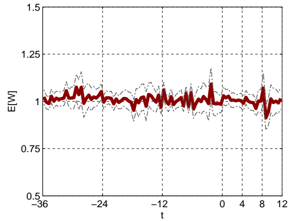
Figure 113: Average waiting time: QoS parameter \beta = 1 .
