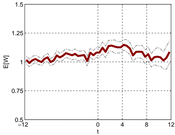
Figure 88: Average waiting time: QoS parameter \beta = 0 .
