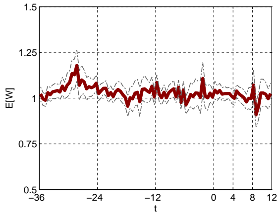
Figure 112: Average waiting time: QoS parameter \beta = 0 .
