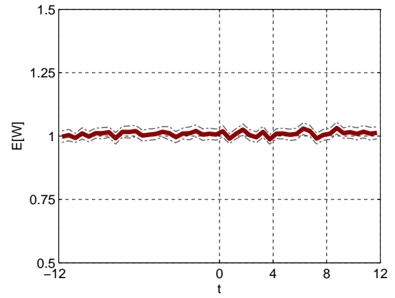
Figure 9: Average waiting time: QoS parameter \beta = 1 .
