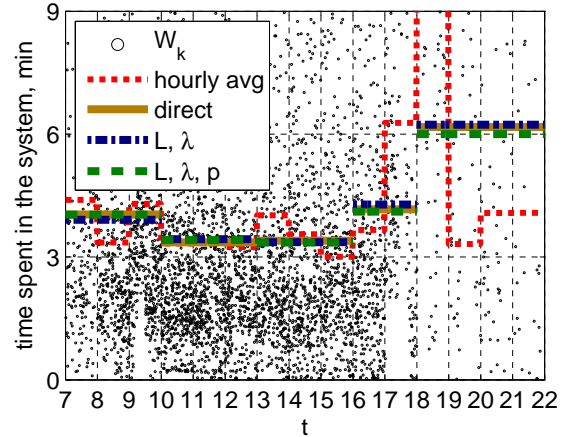
Figure 129: Scatter plot of the waiting times and its hourly averages, \bar{W}(t) , \bar{W}_{L,\lambda}(t) and \bar{W}_{L,\lambda,p}(t) of each hour in [7, 22] on May 4.
