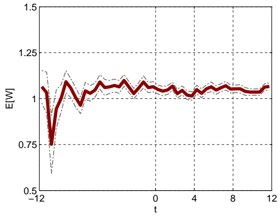
Figure 26: Average waiting time: QoS parameter \beta = 0 .
