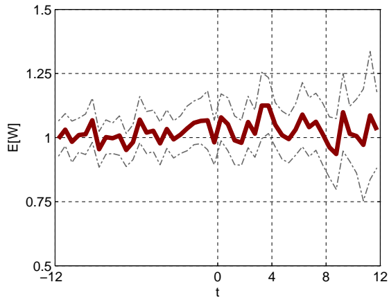
Figure 100: Average waiting time: QoS parameter \beta = 0 .
