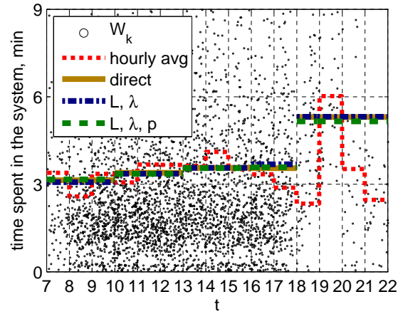
Figure 143: Scatter plot of the waiting times and its hourly averages, \bar{W}(t) , \bar{W}_{L,\lambda}(t) and \bar{W}_{L,\lambda,p}(t) of each hour in [7, 22] on May 17.
