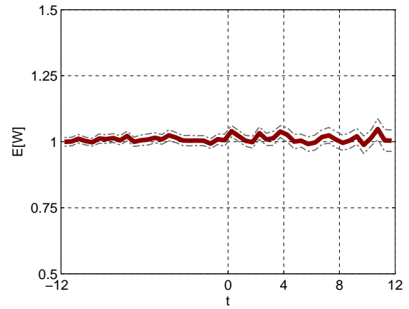
Figure 95: Average waiting time: QoS parameter \beta = 1 .
