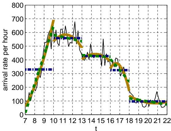
Figure 152: Arrival rate and its approximations by constant, linear and quadratic functions fitted to 5 intervals, [7, 10], [10, 13], [13, 16], [16, 18] and [18, 22], on May 24.
