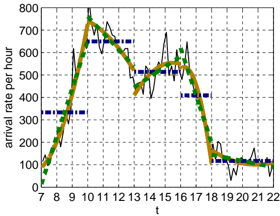
Figure 148: Arrival rate and its approximations by constant, linear and quadratic functions fitted to 5 intervals, [7, 10], [10, 13], [13, 16], [16, 18] and [18, 22], on May 22.
