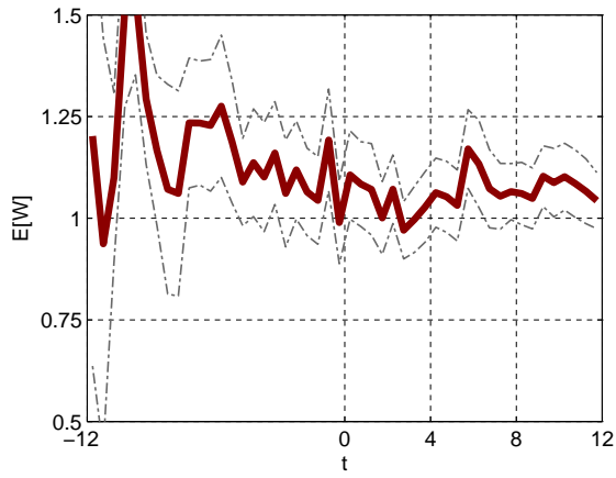
Figure 32: Average waiting time: QoS parameter \beta = 0 .
