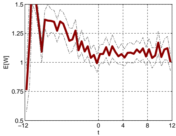
Figure 50: Average waiting time: QoS parameter \beta = 0 .
