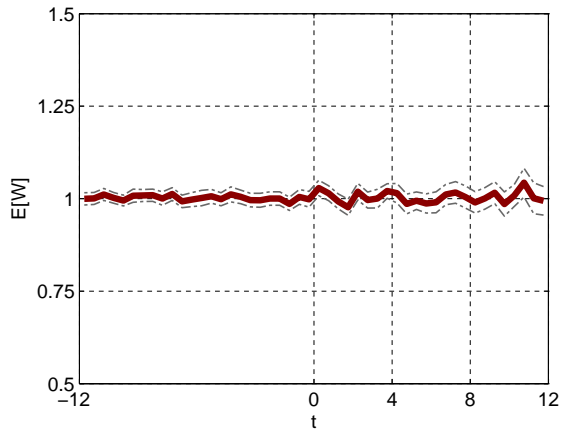
Figure 96: Average waiting time: QoS parameter \beta = 2 .
