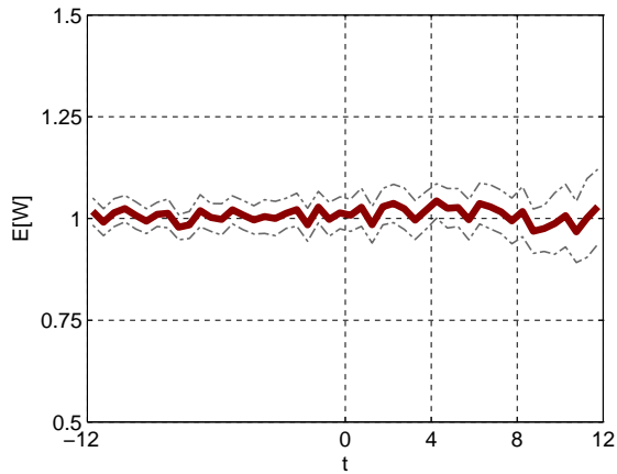
Figure 90: Average waiting time: QoS parameter \beta = 2 .
