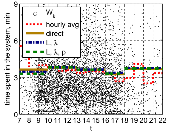
Figure 131: Scatter plot of the waiting times and its hourly averages, \bar{W}(t) , \bar{W}_{L,\lambda}(t) and \bar{W}_{L,\lambda,p}(t) of each hour in [7, 22] on May 7.
