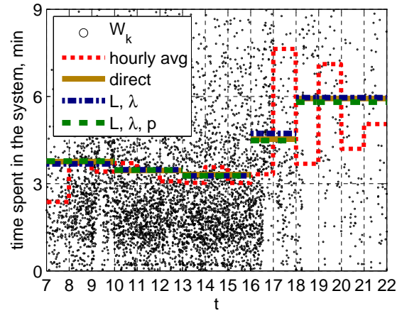
Figure 155: Scatter plot of the waiting times and its hourly averages, \bar{W}(t) , \bar{W}_{L,\lambda}(t) and \bar{W}_{L,\lambda,p}(t) of each hour in [7, 22] on May 25.
