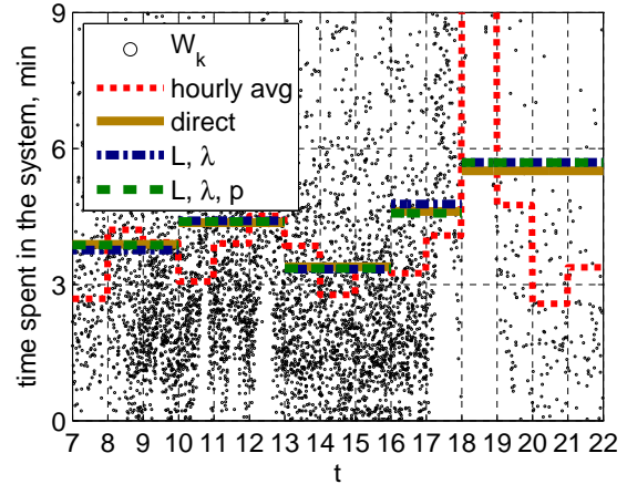
Figure 159: Scatter plot of the waiting times and its hourly averages, \bar{W}(t) , \bar{W}_{L,\lambda}(t) and \bar{W}_{L,\lambda,p}(t) of each hour in [7, 22] on May 30.
