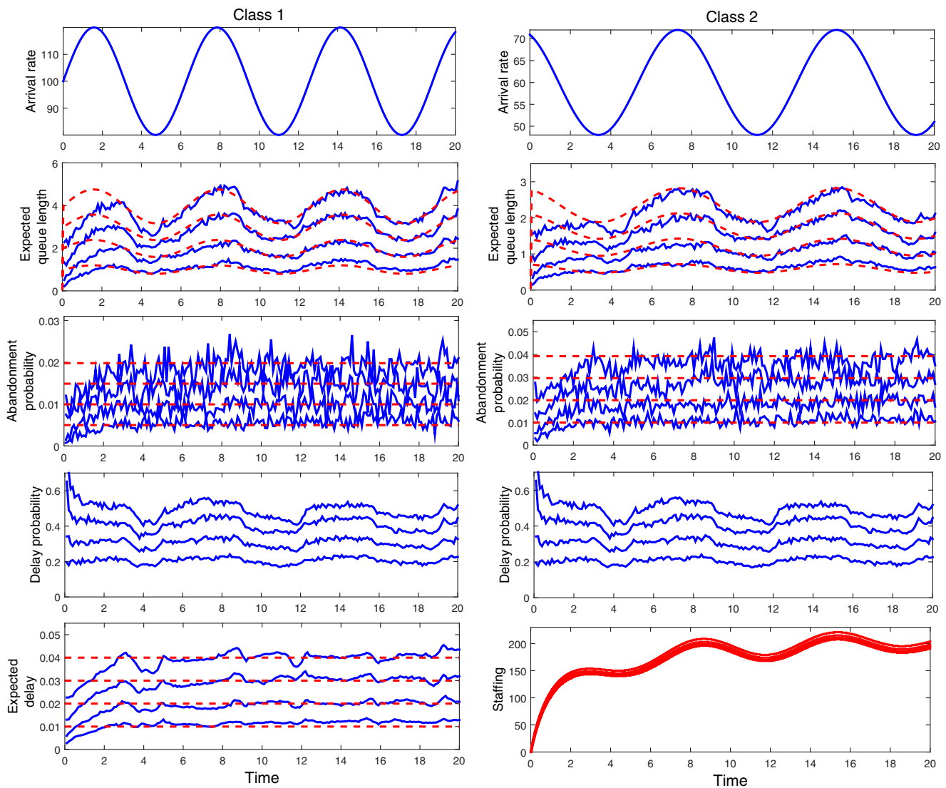
Fig. 6. Performance functions in the \sum_{i=1}^2 (M_t/H_2(m_i, 4) + M(m_i)/s_t) two-class model with the two sinusoidal arrival-rate functions in (22), service-time means m_1 = 1.0 and m_2 = 0.6 and patience means m_1 = 2.0 and m_2 = 1.0 : four cases of identical low waiting-time (high QoS) targets ( w = 0.01, 0.02, 0.03 and 0.04 ) and DIS-MOL staffing at both queues.
