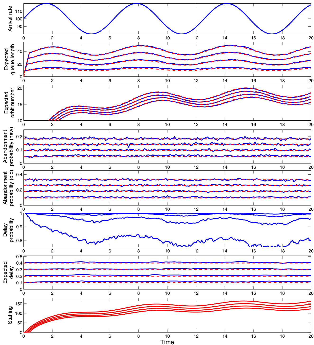
Fig. 2. Performance functions in the (M_r(0.2)/\{H_2(1, 4), H_2(5, 4)\}/s_r + \{M(2), M(1)\}) + (0.2, H_2(1, 4)/\infty) model with the sinusoidal arrival rate in (19) for \bar{\lambda} = 100 and r = 0.2 , Bernoulli feedback with probability p = 0.2 and an IS orbit queue: four cases of high waiting-time (low QoS) targets ( w = 0.10, 0.20, 0.30 and 0.40 ) and simple DIS staffing.
