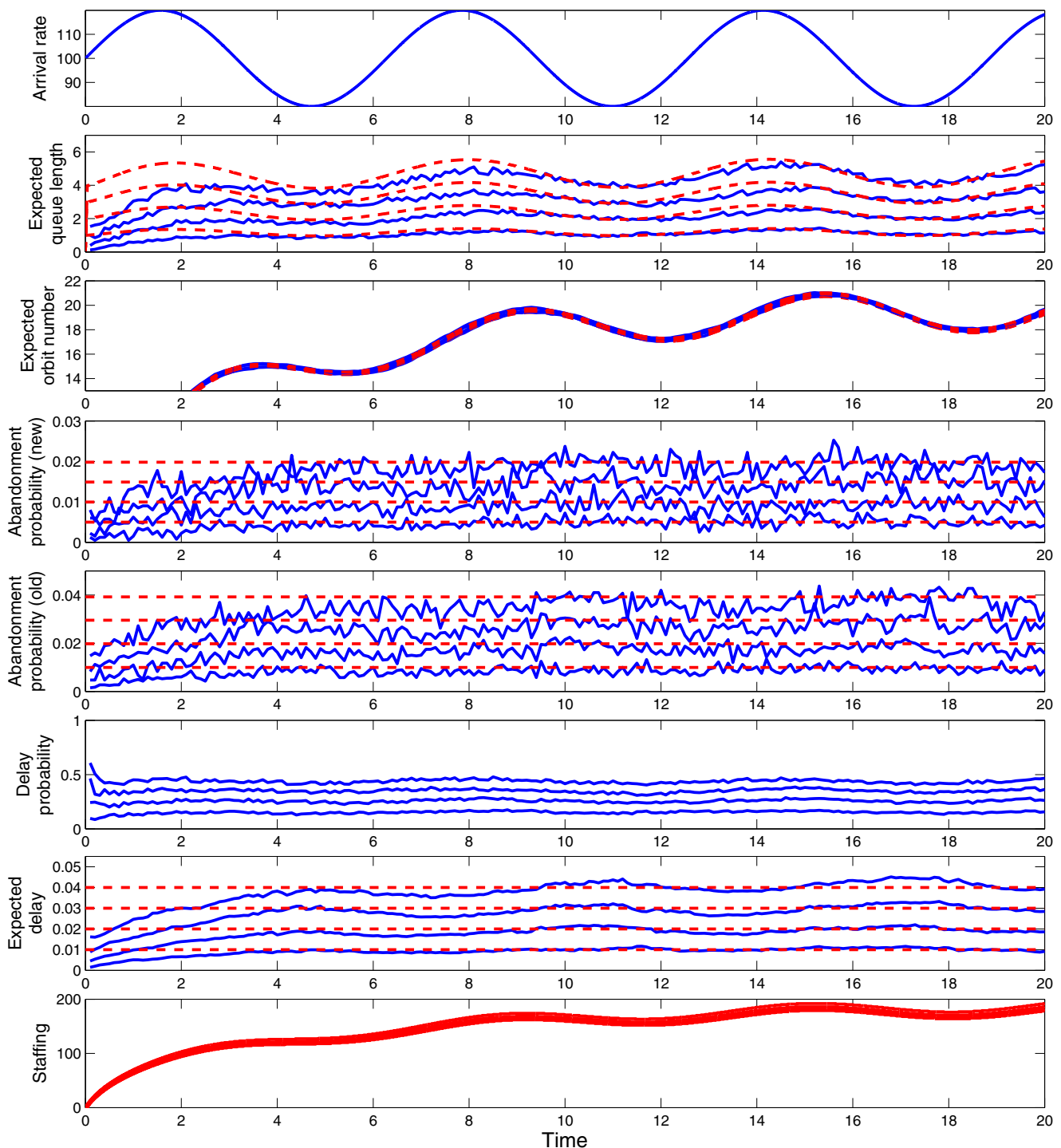
Fig. 3. Performance functions in the (M_t(0.2)/[H_2(1,4), H_2(5,4)]/s_t + \{M(2), M(1)\}) + (0.2, H_2(1,4)/\infty) model with the sinusoidal arrival rate in (19) for \bar{\lambda} = 100 and r = 0.2 , Bernoulli feedback with probability p = 0.2 and an IS orbit queue: four cases of low waiting-time (high QoS) targets ( w = 0.01, 0.02, 0.03 and 0.04 ) and DIS-MOL staffing.
