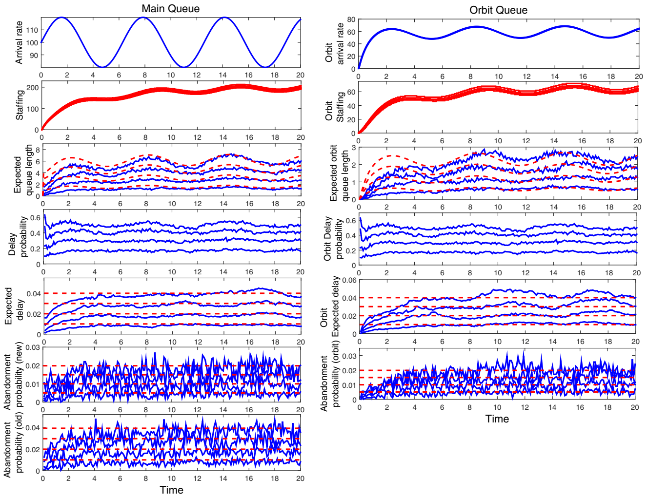
Fig. 8. Performance functions in the (M_r(0.2)/\{H_2(1,4), H_2(10/6,4)\}/s_t + \{M(2), M(1)\}) + (0.6, H_2(1,4)/s_t + M(1)) model with the sinusoidal arrival rate in (19) for \bar{\lambda} = 100 and r = 0.2 , Bernoulli feedback with probability p = 0.6 and an IS orbit queue: four cases of low waiting-time (high QoS) targets ( w = 0.01, 0.02, 0.03 and 0.04 ) and DIS-MOL staffing.
