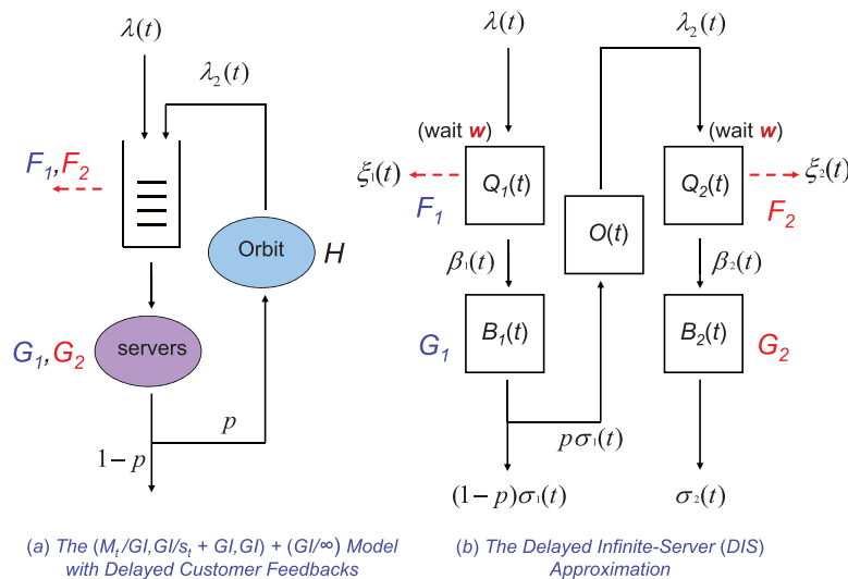
Fig. 1. The (M_t/\{GI, GI\}/s_t + \{GI, GI\}) + (GI/\infty) model with delayed customer feedback and its Delayed Infinite-Server (DIS) approximation. The approximating offered load is m(t) = m_1(t) + m_2(t) = E[B_1(t)] + E[B_2(t)] .
