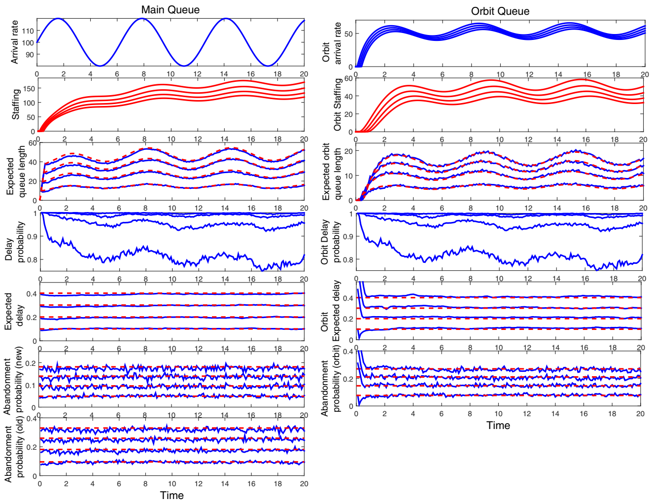
Fig. 7. Performance functions in the (M_t(0.2)/\{H_2(1, 4), H_2(10/6, 4)\}/s_t + \{M(2), M(1)\}) + (0.6, H_2(1, 4)/s_t + M(1)) model with the sinusoidal arrival rate in (19) for \bar{\lambda} = 100 and r = 0.2 . Bernoulli feedback with probability p = 0.6 and a finite-capacity orbit queue: four cases of identical high waiting-time (low QoS) targets ( w = 0.10, 0.20, 0.30 and 0.40 ) and simple DIS staffing at both queues.
