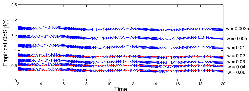
Fig. 4. The empirical Quality of Service (QoS) provided by the DIS-MOL staffing in the (M_t(0.2)/\{H_2(1, 4), H_2(5, 4)\}/s_t + \{M(2), M(1)\}) + (0.2, H_2(1, 4)/\infty) example of Fig. 3 as a function of the waiting-time target w .
