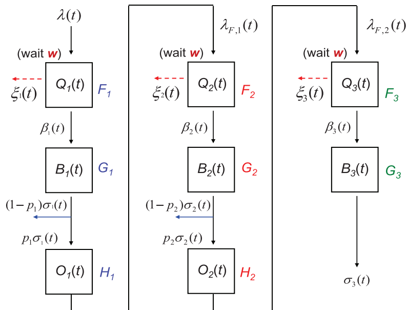
Fig. 9. The DIS approximation for the (M_r/\{GI, GI, GI\}/s_t + \{GI, GI, GI\}) + (GI/\infty) + (GI/\infty) model with two delayed customer feedback opportunities. Here there are two orbit queues. The approximating offered load is m(t) = m_1(t) + m_2(t) + m_3(t) \equiv E[B_1(t)] + E[B_2(t)] + E[B_3(t)] .
