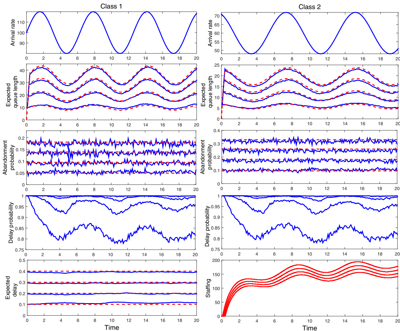
Fig. 5. Performance functions in the \sum_{i=1}^2 (M_i/H_2(m_i, 4) + M(m_i)/s_i) two-class model with the two sinusoidal arrival-rate functions in (22), service-time means m_1 = 1.0 and m_2 = 0.6 and patience means m_1 = 2.0 and m_2 = 1.0 : four cases of identical high waiting-time (low QoS) targets ( w = 0.10, 0.20, 0.30 and 0.40 ) and simple DIS staffing at both queues.
