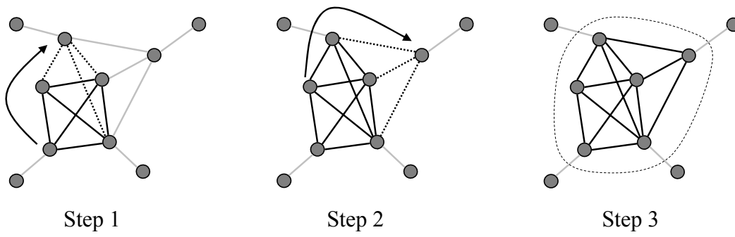
Figure 5: Illustrating the logic of the CPM algorithm
