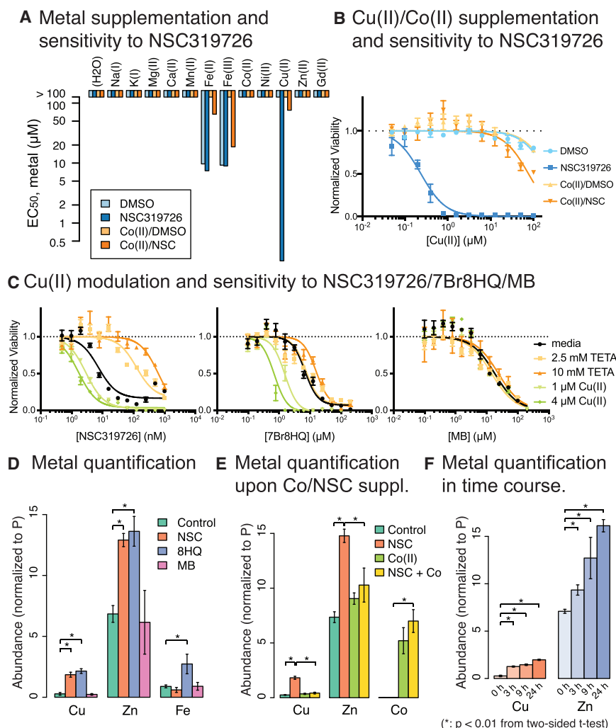
Figure 3. NSC319726 Induces Copper Toxicity
