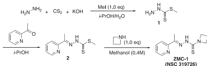
Scheme 1: Synthesis of NSC319726
