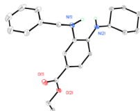
Figure 5. SAR study of Fer-1. (a) EC 50 , cLogP, and % DPPH inhibition of selected potent ferrostatins. DPPH: 2,2-diphenyl-1-picrylhydrazyl radical. (b) X-ray structure of the most potent Fer-1 analogue (SRS11-92).
