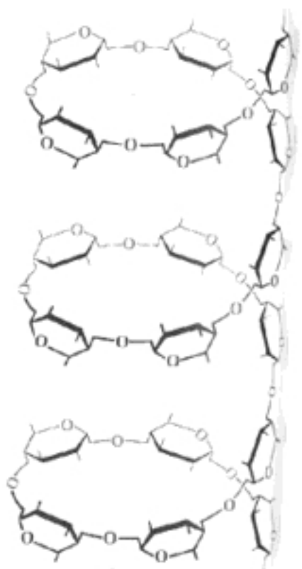
Part of a helical starch chain
