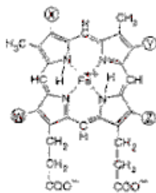
Heme
