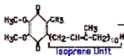
Ubiquinone
