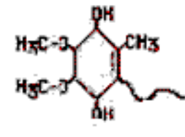
Ubiquinol
