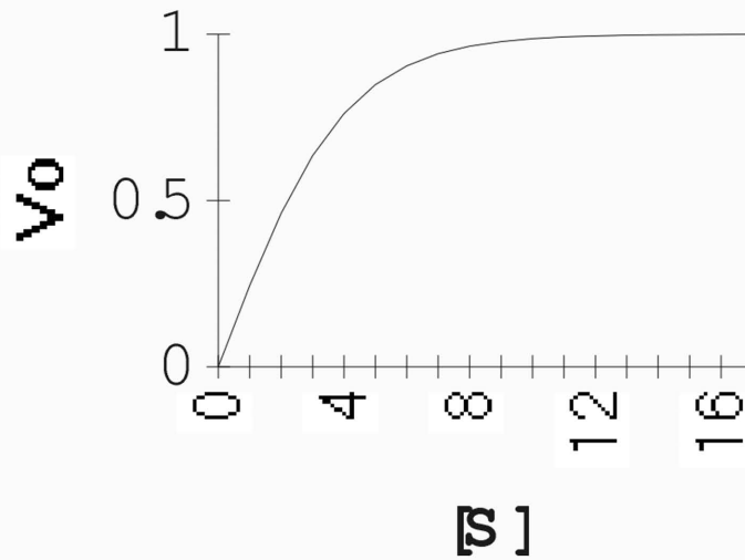
Michaelis-Menton Graph
