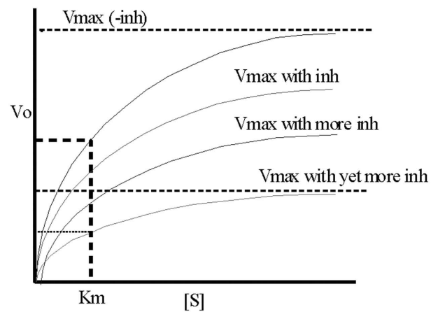
Non-competitive inhibition
