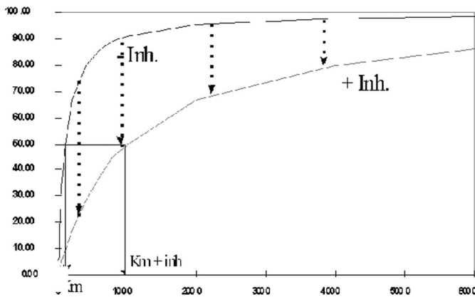
Competitive inhibition
