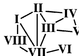
Scheme 1: Connections between Helices via Hydrogen Bonding a
