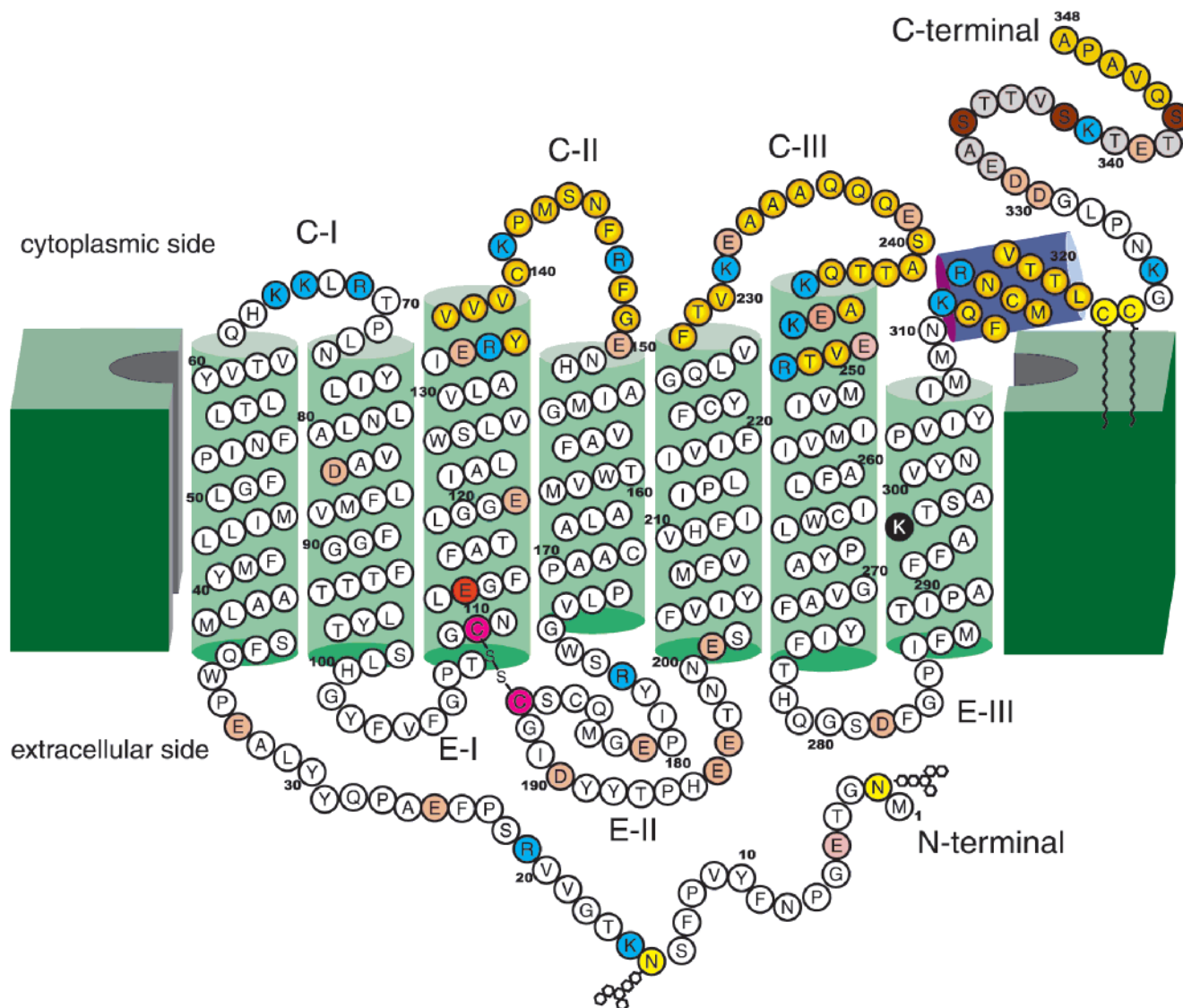
FIGURE 2: Two-dimensional model of bovine rhodopsin adopted after that of Hargrave (9). About \frac{1}{4} of the polypeptide chain of opsins has cytoplasm exposure; \frac{1}{4} is sequestered in the intradiscal space, and \frac{1}{2} forms a core of transmembrane helices. Green cylinders represent helices that in large part are imbedded in the disk membranes (19–34 residues each). The violet cylinder represents the amphiphilic helix (H-VIII) that runs parallel to the membranes. The color of rhodopsin results from the protonated Schiff base linkage of the 11- cis -retinal chromophore (100). Lys 296 forms this protonated Schiff base with retinal and is shown as a black filled circle. Glu 113 is a counterion of the Schiff base and is shown as a red filled circle. The disulfide bridge conserved among GPCRs is shown as purple filled circles (60). Two carbohydrate moieties at Asn 2 and Asp 15 and two palmitoyl groups at Cys 322 and Cys 323 (15, 64–71) are shown as light yellow filled circles (32, 72, 73). Light red filled circles represent acidic residues, and blue filled circles represent basic residues. Photoisomerization of the 11- cis -retinal chromophore of rhodopsin to all-trans -retinal leads to a conformational change in the protein, including the cytoplasmic surface (9–14, 32, 118, 119) leading to activation of G i . Loops CII and CIII and helix VIII are involved in the recognition of G i and are marked with filled yellow circles at the center, changing to red filled circles in the periphery. These residues are also important in binding of two regulatory proteins: rhodopsin kinase and arrestin. The functional phosphorylation occurs in the C-terminal region (represented by light brown filled circles) at phosphorylation sites denoted by dark brown filled circles (86–91, 96). The last five C-terminal residues were postulated to be involved in the vectorial transport within highly differentiated rod photoreceptors (92, 93, 120). The carbohydrate chains and the disulfide linkage (in pink filled circles) are oriented toward the lumen (extracellular) face of rhodopsin, and the C-terminal domain is cytoplasmic. To date, more than 100 mutations in the human rhodopsin gene have been associated with recessive and dominant retinitis pigmentosa (RP), as well as congenital stationary night blindness (CSNB).
