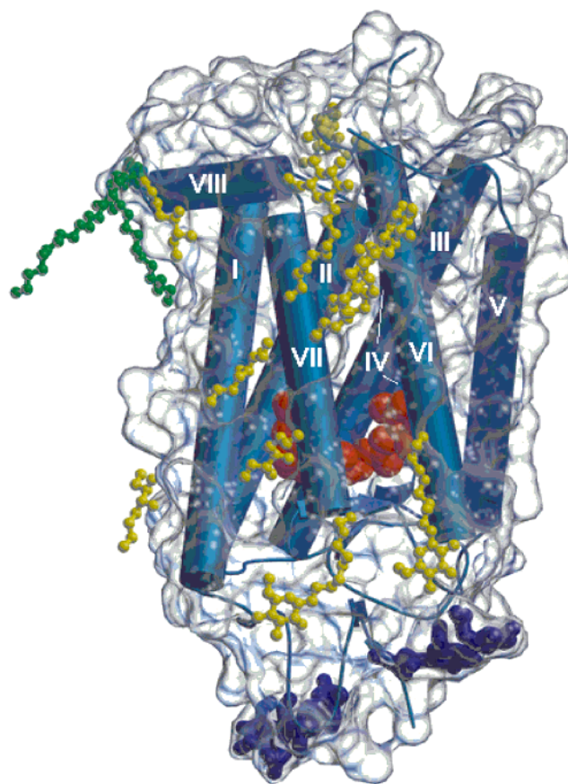
FIGURE 1: Three-dimensional crystal structure of rhodopsin with bound detergent and amphiphile molecules. Helical portions of the protein, including the seven transmembrane helices, are shown as blue rods, and \beta -strands are shown as blue arrows. The polypeptide connecting the helices appears as blue coils. A transparent envelope around the protein represents the molecular surface. The dark blue ball-and-stick groups at the bottom of the figure denote carbohydrate groups attached to the protein. Two palmitoyl groups covalently attached to the protein are shown in green. Nonylglucoside and heptanetriol molecules located near the hydrophobic surface of the protein are shown in yellow. The figure was drawn using Molscript (116) and Raster3d (117).
