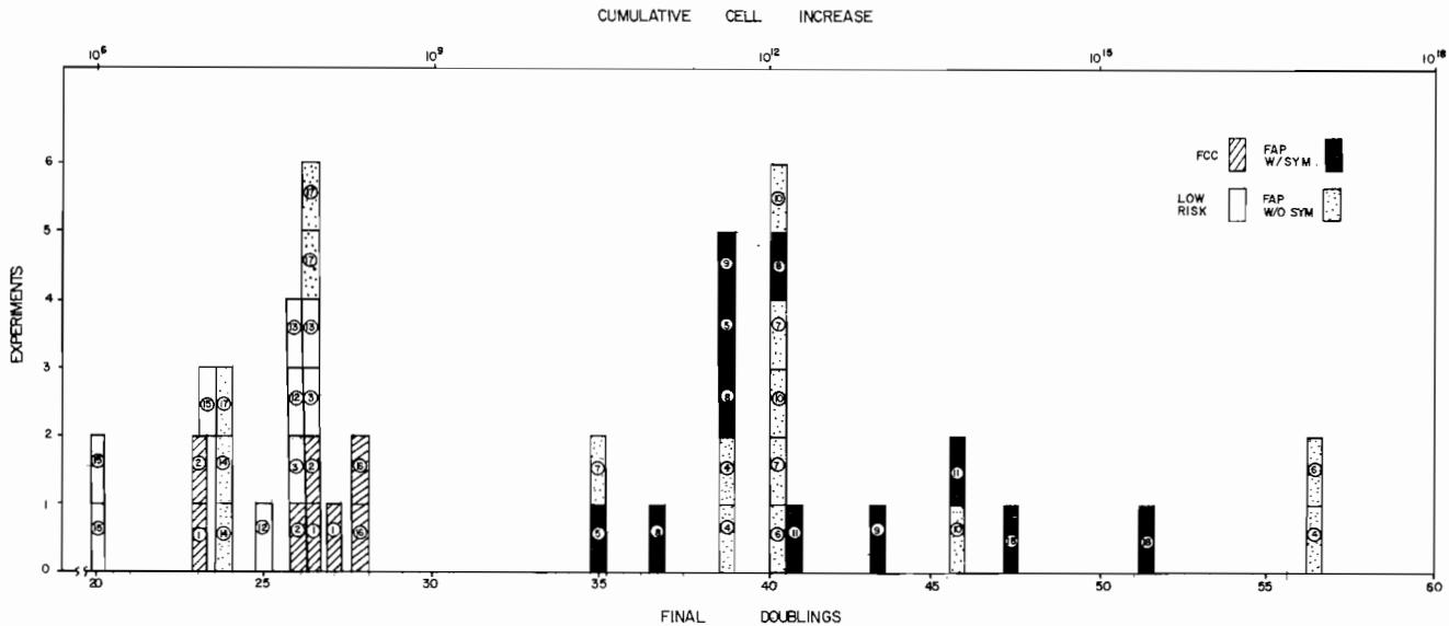
FIG. 2. Distribution of last doublings for human skin fibroblast lines passed by the 3T3 protocol. Each box is a separate experiment. Cell lines are indicated by numbers as listed in Table 3.
