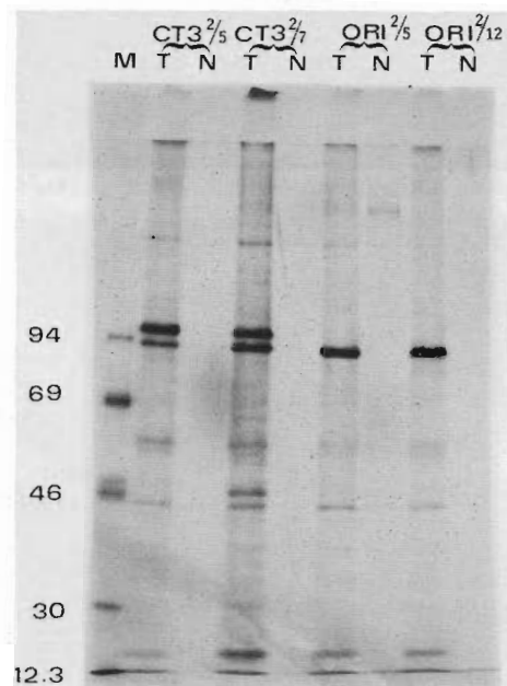
FIG. 3. Autofluorogram of immunoprecipitations of [ 35 S]methionine-labeled cell extracts from pSVCT3-2/5, pSVCT3-2/7, pSVRIori-minus-2/5, and pSVRIori-minus-2/12 human transformants. T, Tumor serum; N, normal serum. Numbers indicate the sizes (in kilodaltons) of protein markers.
