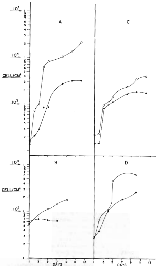
FIG. 2. Growth properties of pSVRIori-minus- and pSVCT3-transformed cells. (A) SV101-SV40-transformed Swiss 3T3 mouse cells; (B) CCDSK141 normal human cells; (C) pSVRIori-minus-transformed CCDSK141 cells; (D) pSVCT3-transformed CCDSK141 cells. O, 10% serum; ●, 1% serum.
