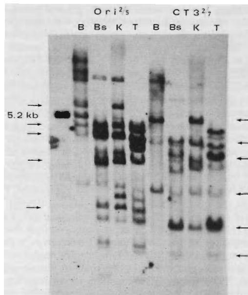
FIG. 4. Southern blot analysis of ori-minus-2/5 and pSVCT3-2/5 human transformants. DNA was cut with restriction enzymes that cut SV40 in only one place. B, BclI ; Bs, BstXI ; K, KpnI ; T, TaqI . Arrows indicate partial repeats (see Materials and Methods). kb, Kilobases.
