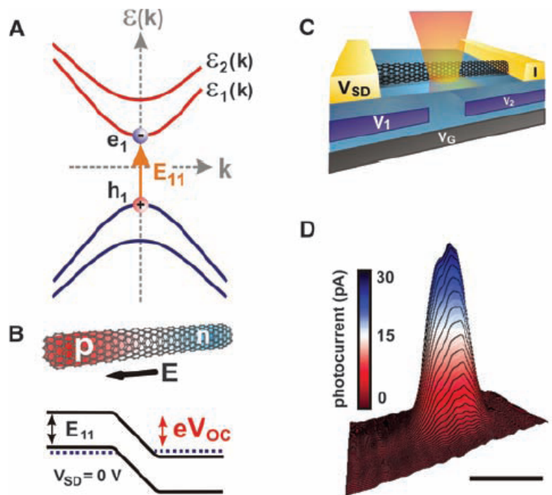
Fig. 1. Band structure, device geometry, and spatial photocurrent of the carbon nanotube p-n junction photodiode. (A) Electronic band structure diagram of the carbon nanotube showing electron-hole pair creation into the first subband \epsilon_1 of the nanotube. e_1 labels the electron (blue) and h_1 labels the hole (red) of masses m_1^* . (B) (Top) Schematic of the carbon nanotube showing p-type (positive, red) and n-type (negative, blue) regions with built-in electric field E . (Bottom) Length-dependent potential energy diagram of p-n junction at V_{SD} = 0 V. Dotted lines represent the electron Fermi energy in the p- and n- type regions of the device,
