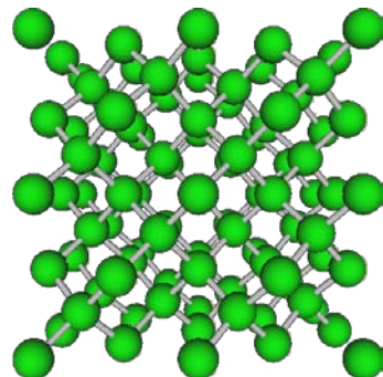
Silicon Nanocrystal
