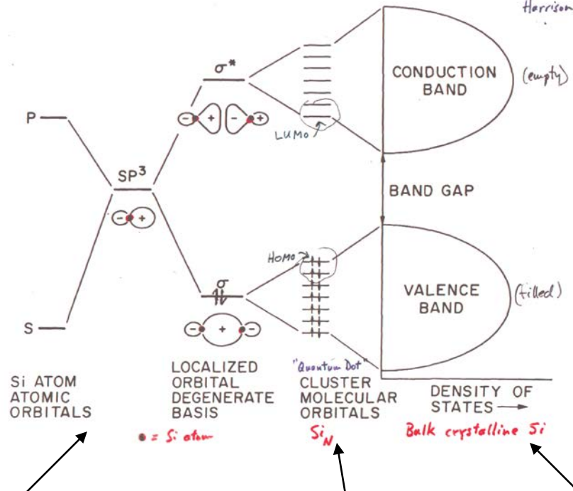
MOLECULAR ORBITAL MODEL FOR SEMICONDUCTOR BAND STRUCTURE
