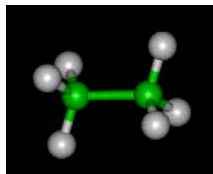
Disilane molecule
