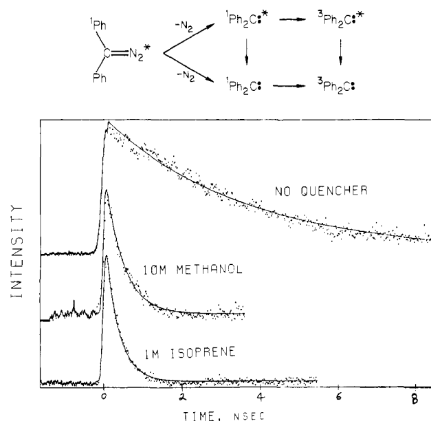
Figure 1. Decay curves of excited triplet diphenylcarbene with no quencher, 10 M methanol, and 1 M isoprene in degassed acetonitrile at room temperature. The points are experimental, and the solid curves are theoretical.
