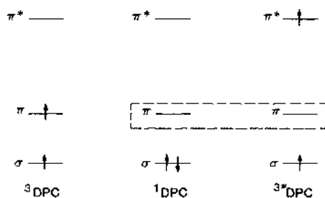
Fig. 5. Orbital occupancy for ^3\text{DPC} (ground state), ^1\text{DPC} (low-energy singlet state), and ^3\text{DPC} (excited state of ^3\text{DPC} ). Note the empty, low-energy \pi orbital common to ^1\text{DPC} and ^3\text{DPC} .
