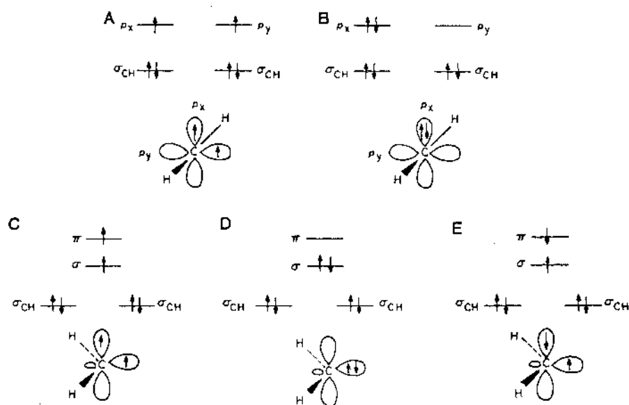
Fig. 2. Energy level and orbital representations for bent and linear geometries of methylene. (A) Linear methylene, the triplet state. (B) Linear methylene, the singlet state. (C) Bent methylene, the triplet state, (\sigma)^1(\pi)^1 . (D) Bent methylene, the singlet state, (\sigma)^2 . (E) Bent methylene, the high-energy singlet state, (\sigma)^1(\pi)^1 .
