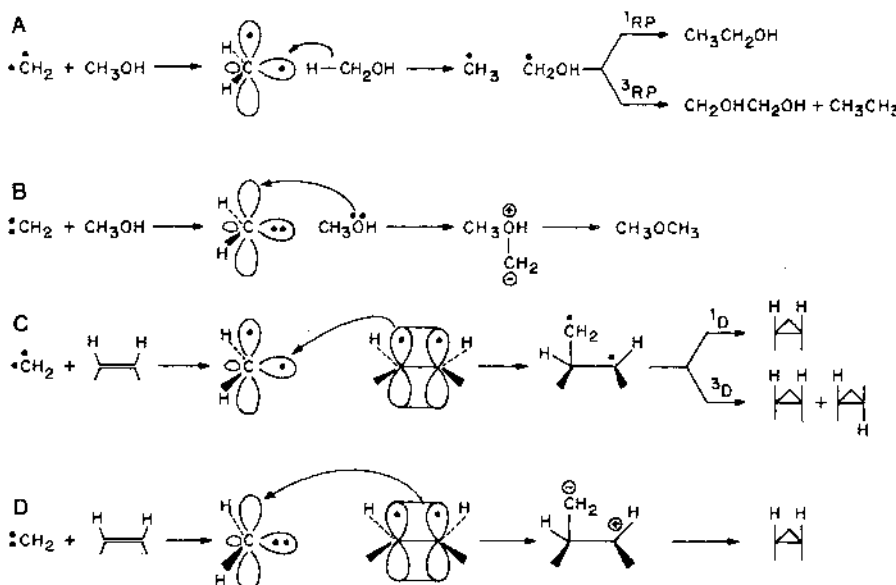
Fig. 3. Some prototypical reactions of divalent carbon with methylene as an example. RP and D represent radical pairs and diradicals, respectively. A superscript 1 stands for a singlet state; a superscript 3, a triplet state.
