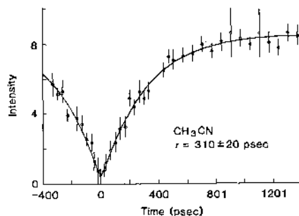
Fig. 4. Laser-induced fluorescence as a function of time delay between excitation and probe pulses yielding ^1\text{DPC} \rightarrow ^3\text{DPC} for diphenylcarbene in acetonitrile.
