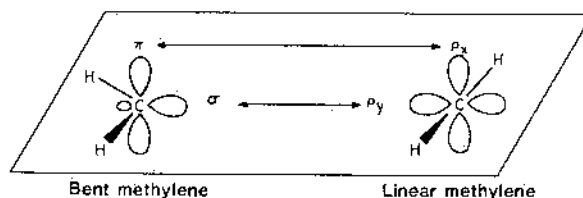
Fig. 1. Orbital representations for bent and linear methylenes. For bent methylene, the hydrogen atoms and the \sigma orbital are in the indicated plane; the \pi orbital is above and below it. For linear methylene, the hydrogen atoms and the p_y orbital are in the plane; the p_x orbital is above and below it.
