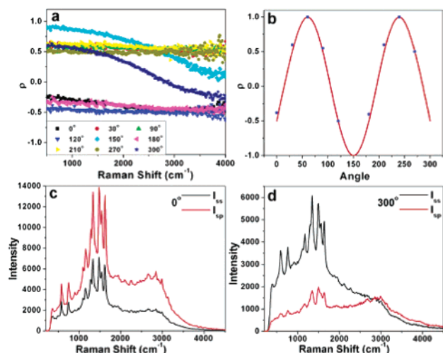
Figure 5. Simultaneous measurement of s- and p-polarized SERS signals from a single R6G molecule on an Ag aggregate. 528.7 nm laser excitation was used with a fixed intensity of \sim 80 W/cm 2 . (a) Raman shift dispersion of polarization parameter \rho (see text) at various rotation angles. (b) Averaged \rho at various angles fitted with a \cos(2\theta) curve. (c and d) Raman spectra for the two different behaviors, constant \rho and varying \rho as a function of Raman shift, respectively.
