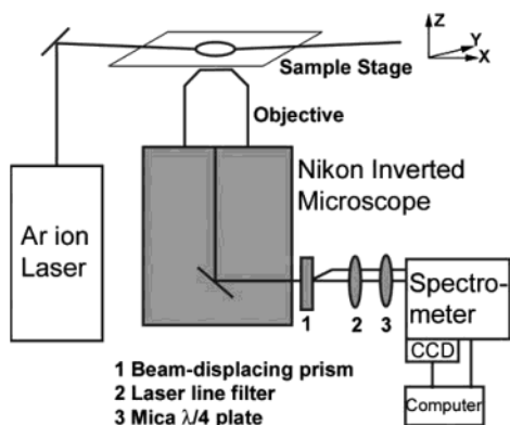
Figure 4. Schematics of the experimental setup. s- and p-scattered light is displaced by a beam displacing prism and simultaneously recorded on a CCD camera.
