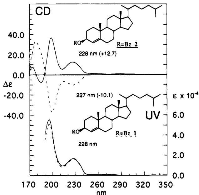
Figure 1. CD and UV spectra of cholest-4-en-3 \beta -ol benzoate ( 1 ) and cholest-4-en-3 \alpha -ol benzoate ( 2 ), in hexane.
