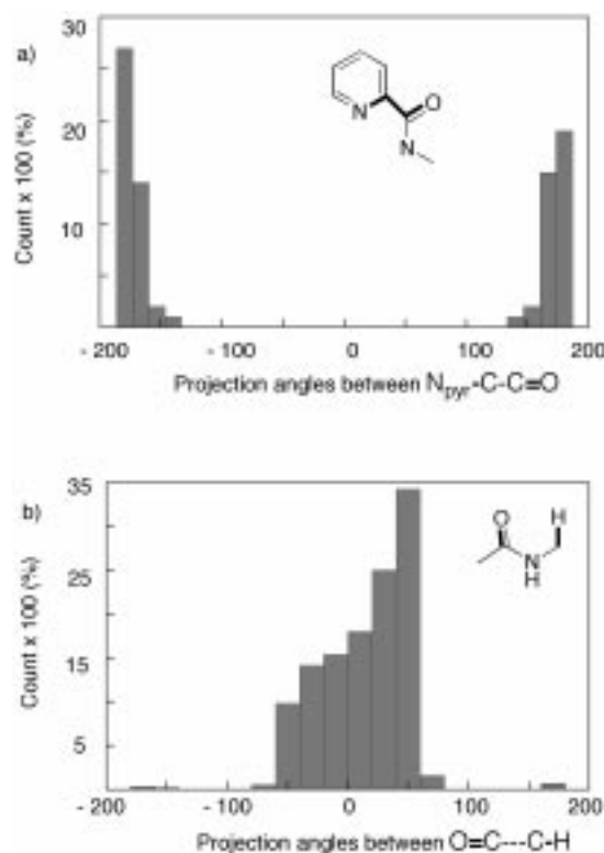
Figure 4. a) Projection angle ( \text{N}_{\text{pyr}}-\text{C}-\text{C}=\text{O} ) distribution in crystal structures of compounds containing pyridine-2-carboxamide in Cambridge Structural Database. b) Projection angle ( \text{O}=\text{C}-\text{C}-\text{H} ) distribution in crystal structures of compounds containing secondary amide in Cambridge Structural Database.
