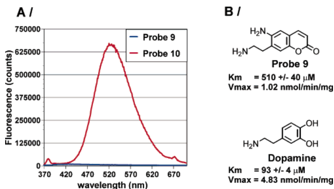
Figure 3. (A) Emission spectra of probes 9 and 10 ( 5 \mu\text{M} , pH 7.4, \lambda_{ex} = 335 nm). (B) Kinetic parameters for probe 9 and dopamine (MAO B).
