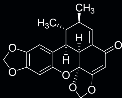
carpanone
