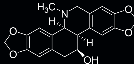
chelidonine
