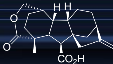
gibberelline A 15
