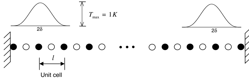
Fig. 1. An atomic chain and a unit cell.
