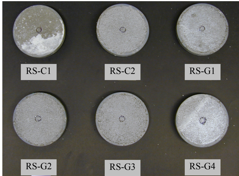
Fig.7 Typical cracking patterns of slabs after punching shear (top face) (For description of specimen IDs refer to table 2.)
