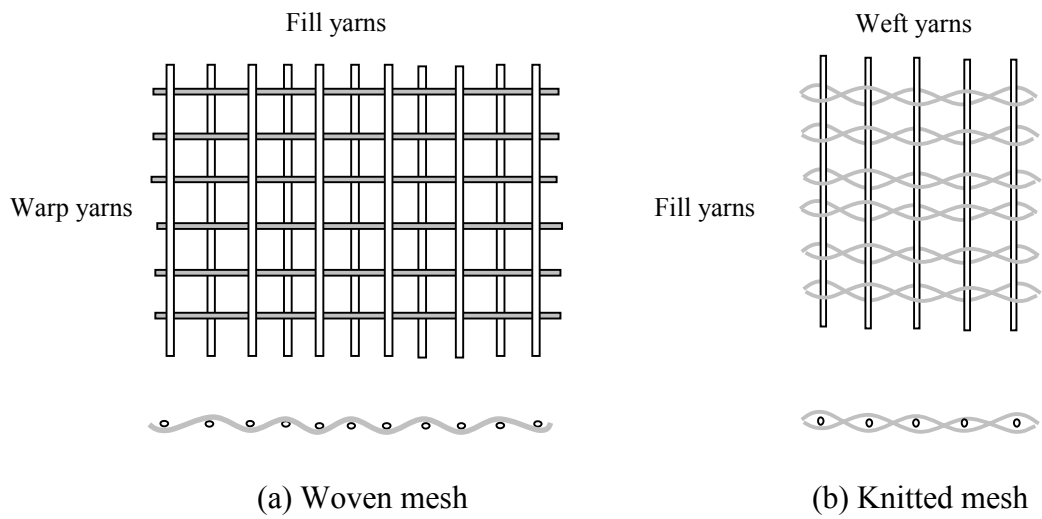
Fig.1 Structures of fabric mesh
