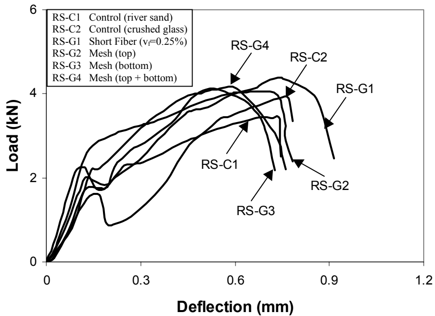
Fig.6 Load-deflection curves for slabs in punching shear
