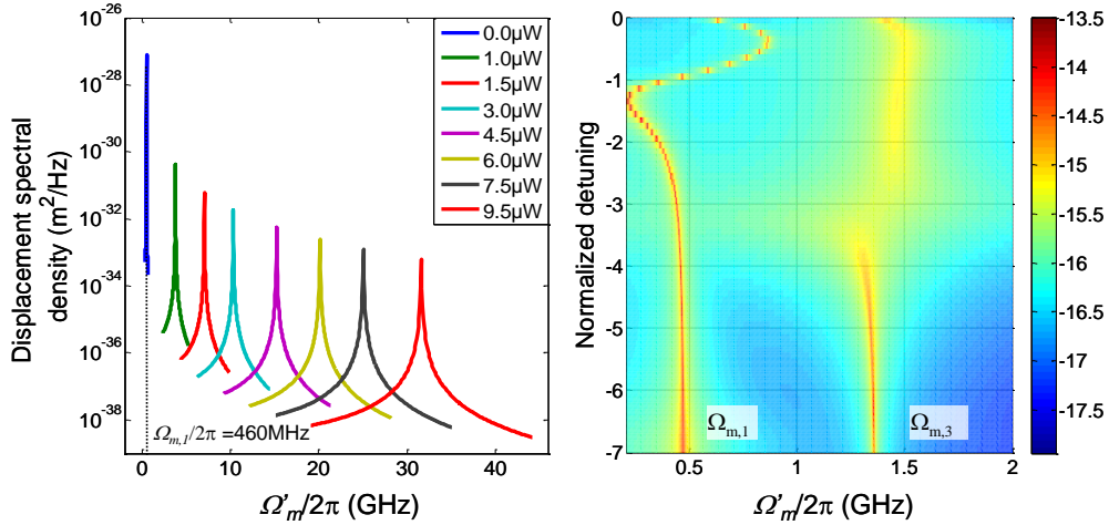
Fig. 7. (a) Displacement spectral density of the first mechanical mode, with optical detuning from the first optical mode. With the input power increasing from 0 to 9.5 μW, in addition to an observed optical stiffening, the amplitude decreases with a larger linewidth for a decrease in the effective temperature. The detuning \Delta\tau is fixed at -0.25 , for an optical Q of 5 \times 10^5 , m_{\text{eff}} of 200 fg, at 300 K bath temperature. (b) Displacement spectral density of the first and second allowed mechanical modes with different detunings. The scale bar is in dB with units of m 2 /Hz (pump powers P_1 of 0.1 μW and P_2 of 50 μW used respectively in the modeling).
