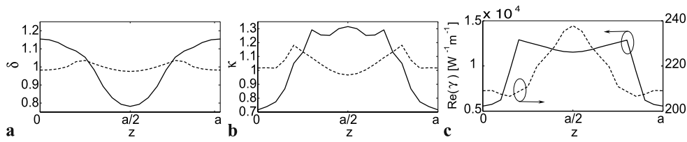
Fig. 2 The group-velocity shift \delta , the mode overlap parameter \kappa , and waveguide nonlinear coefficient \gamma vs. distance z , calculated for the fast- and slow-light modes presented in Fig. 1(c). Dashed and solid curves correspond to the fast- and slow-light modes, respectively
