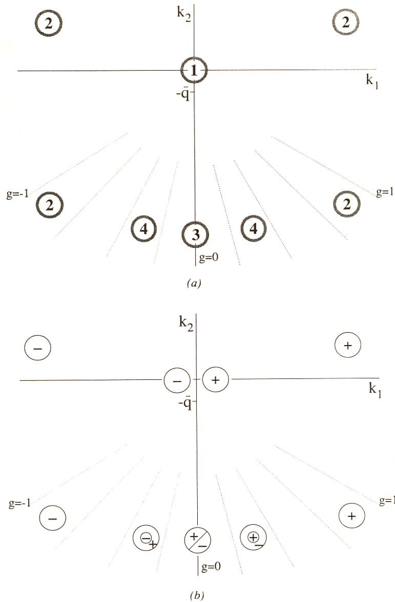
Figure 10. Four principal parameter regimes. (a) The four regimes for a general covariance matrix \mathbf{Q} . (b) The regimes for Linsker's layer \mathcal{B} \rightarrow \mathcal{C} connections. See text for explanation of the regimes. When k_2 is large and negative, the DC constraint is approximately constant along the radial lines of constant k_1/(k_2 + \bar{q}) , so each of the parameter regimes with large negative k_2 is wedge shaped. From [6].
