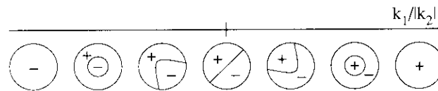
Figure 2. Linsker's results at layer C . Each circle represents the spatial pattern of inputs from layer B to a cell in layer C that resulted from a given choice of k_1/|k_2| , for k_2 large and negative. As the parameter k_1 was varied, synaptic structures ranging from saturated structures through centre-surround structures to bi-lobed oriented structures were reported.
