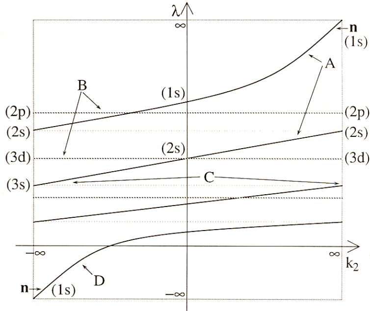
Figure 6. General spectrum of eigenvalues of \mathbf{Q} + k_2\mathbf{J} as a function of k_2 . A: Eigenvectors with non-zero DC component (solid lines) vary with k_2 , and have eigenvalues that increase monotonically with k_2 . B: Eigenvectors with zero DC component (thick dotted lines) are independent of k_2 . C: Adjacent DC eigenvalues share a common asymptote (thin dotted lines). D: There is only one negative eigenvalue. The leading eigenvector at k_2 = \infty and the negative eigenvector at k_2 = -\infty are both equal to the DC vector, \hat{n} . The annotations in parentheses identify the eigenvectors of Linsker's system at layer \mathcal{B} \rightarrow \mathcal{C} . From [6].
