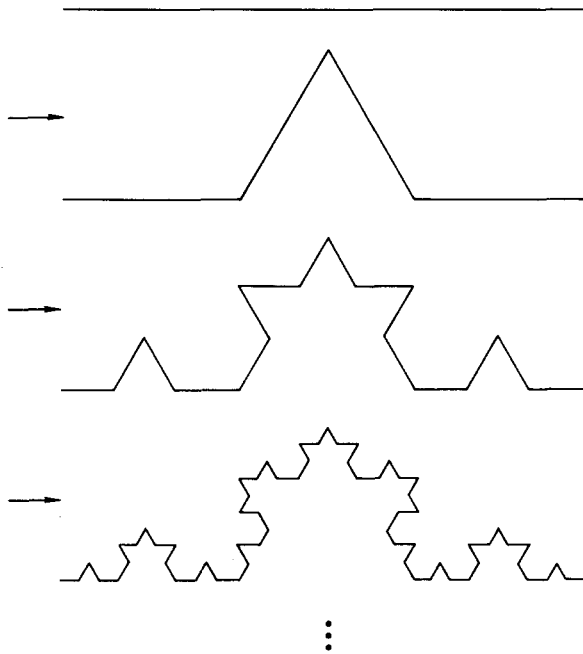
Fig. 1. Construction of the Koch curve.
