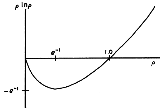
FIG. 1. A graph of \rho \ln \rho versus \rho for real values of \rho .
