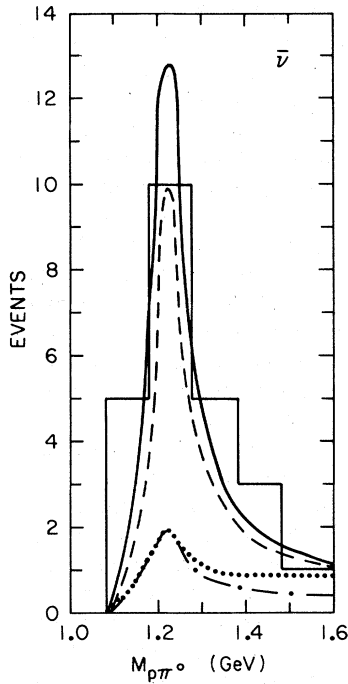
FIG. 7. Same as Fig. 6 but for the process \bar{\nu}p \rightarrow \bar{\nu}p\pi^0 .
