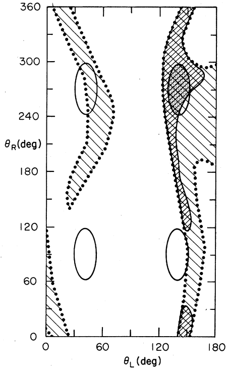
FIG. 2. The allowed angles in the coupling planes of Fig. 1 for fixed radii taken at the center of the allowed annulus ( r_L = 0.53 ) in the left-coupling plane and at the outer edge of the allowed annulus ( r_R = 0.22 ) in the right-coupling plane. The ellipses indicate the regions allowed by inclusive pion data; going clockwise from the upper-right they are regions A, B, C, and D, respectively. The area shaded with lines and enclosed with a dotted curve is allowed by elastic data. The region which is cross hatched is allowed by elastic and exclusive-pion results. The area shaded with dots is the only region allowed by all data.
